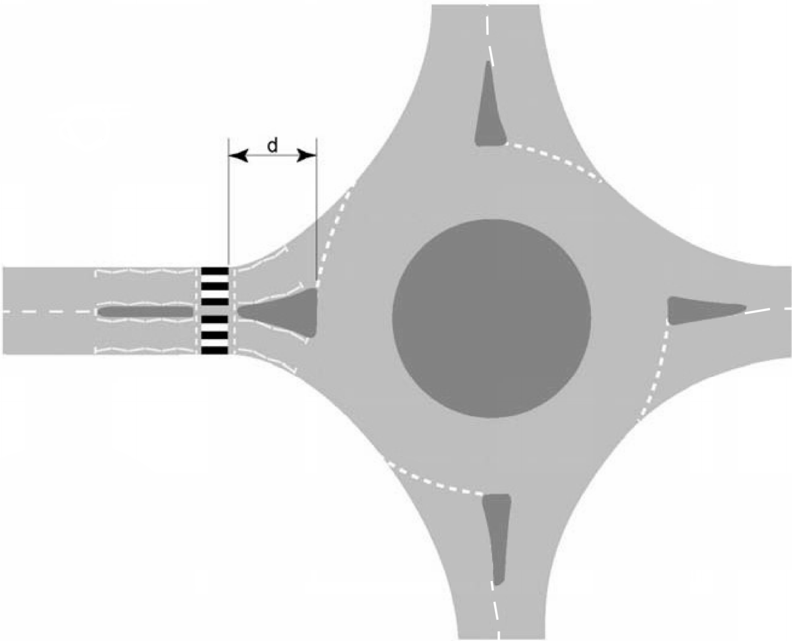
Figure 8.1.4 Measurement of distance from roundabout to pedestrian crossing
