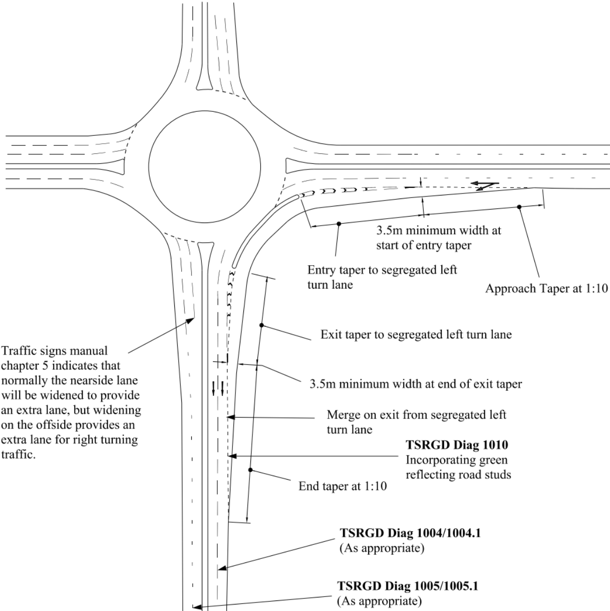
Figure 6.27N2b Diverge/merge layout SLTL island <50 metres in length
