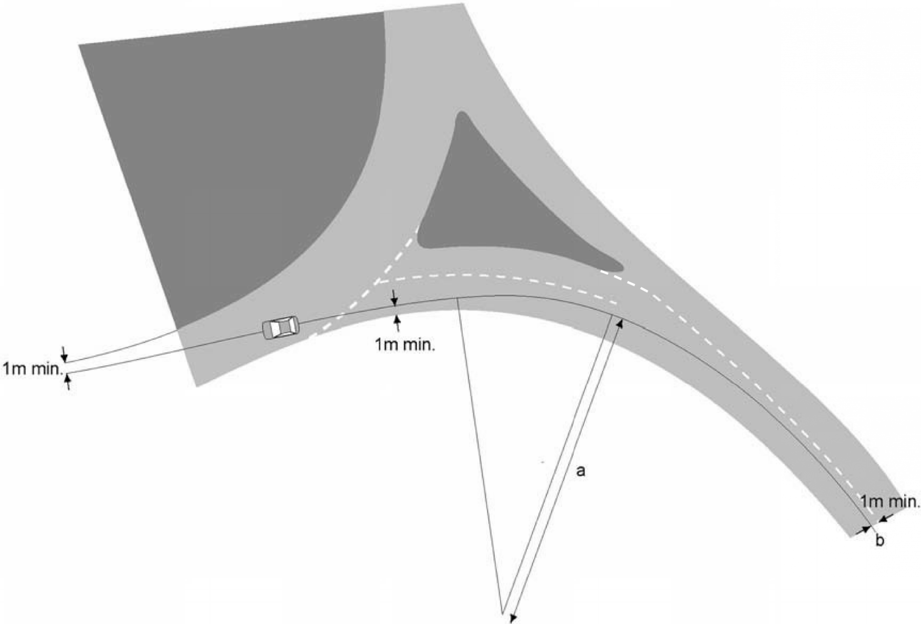
Figure 3.22 Determination of entry path radius for the left turn where the approach curves to the left
