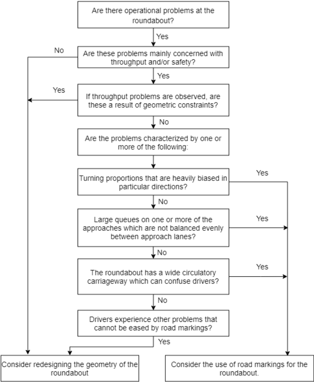
Figure D.1 Chart illustrating general principles
