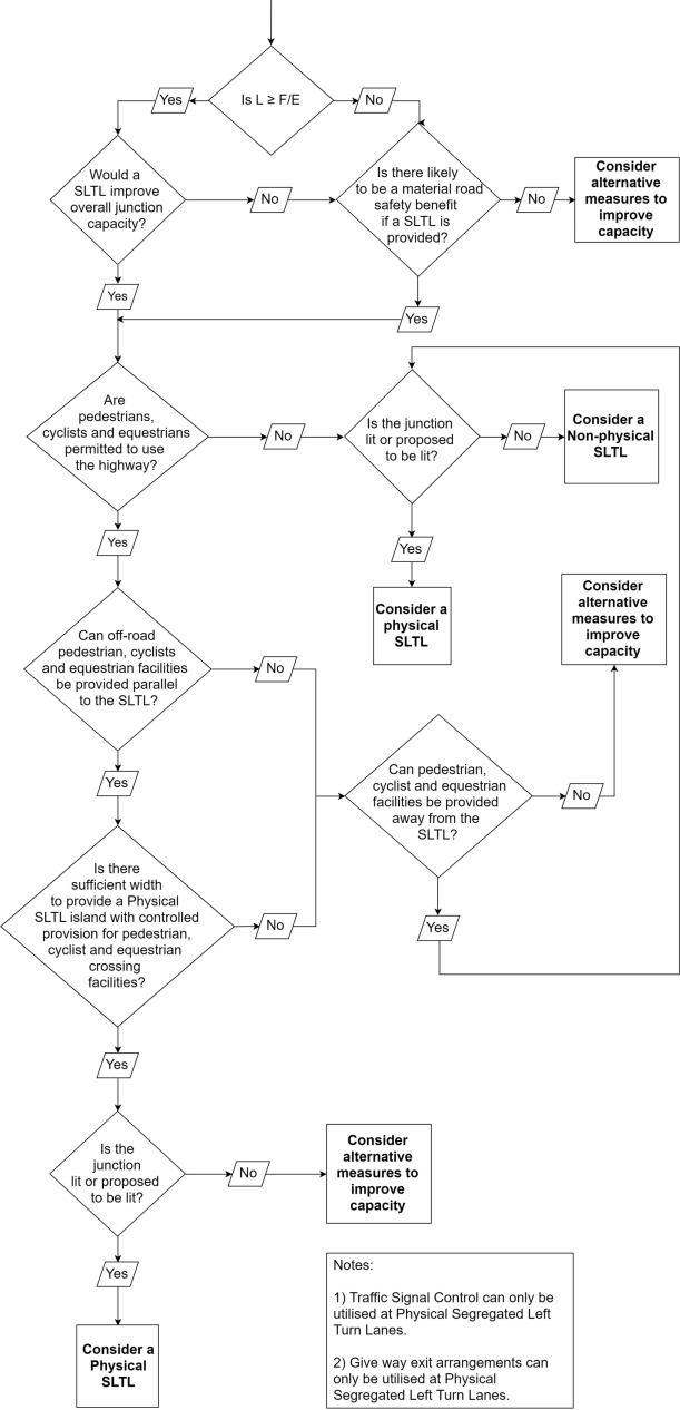
Figure C.1 Example of flow chart decision process for incorporation of SLTL
