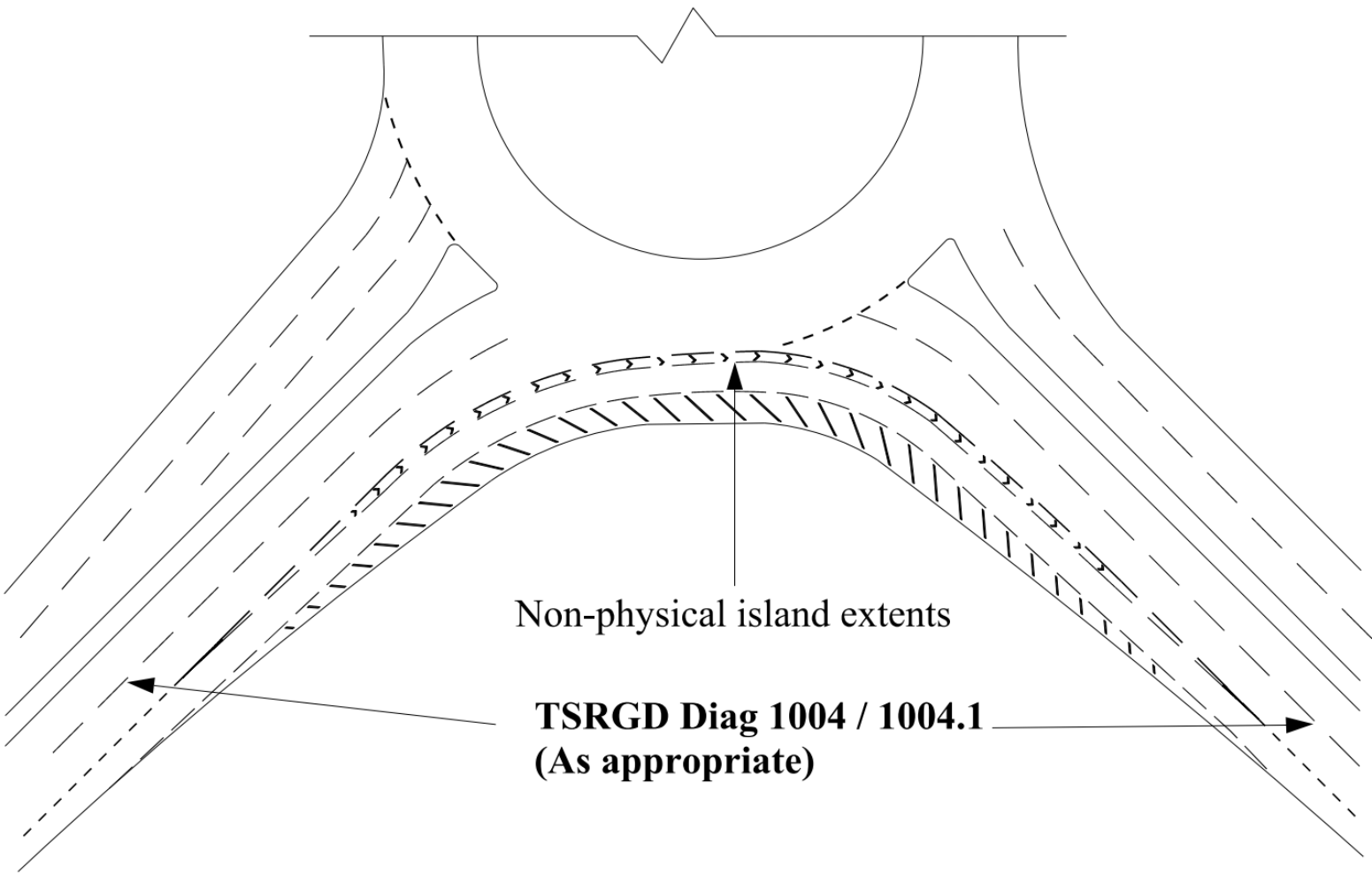
Figure 6.53.2a Generic non-physical segregated left turn lane
