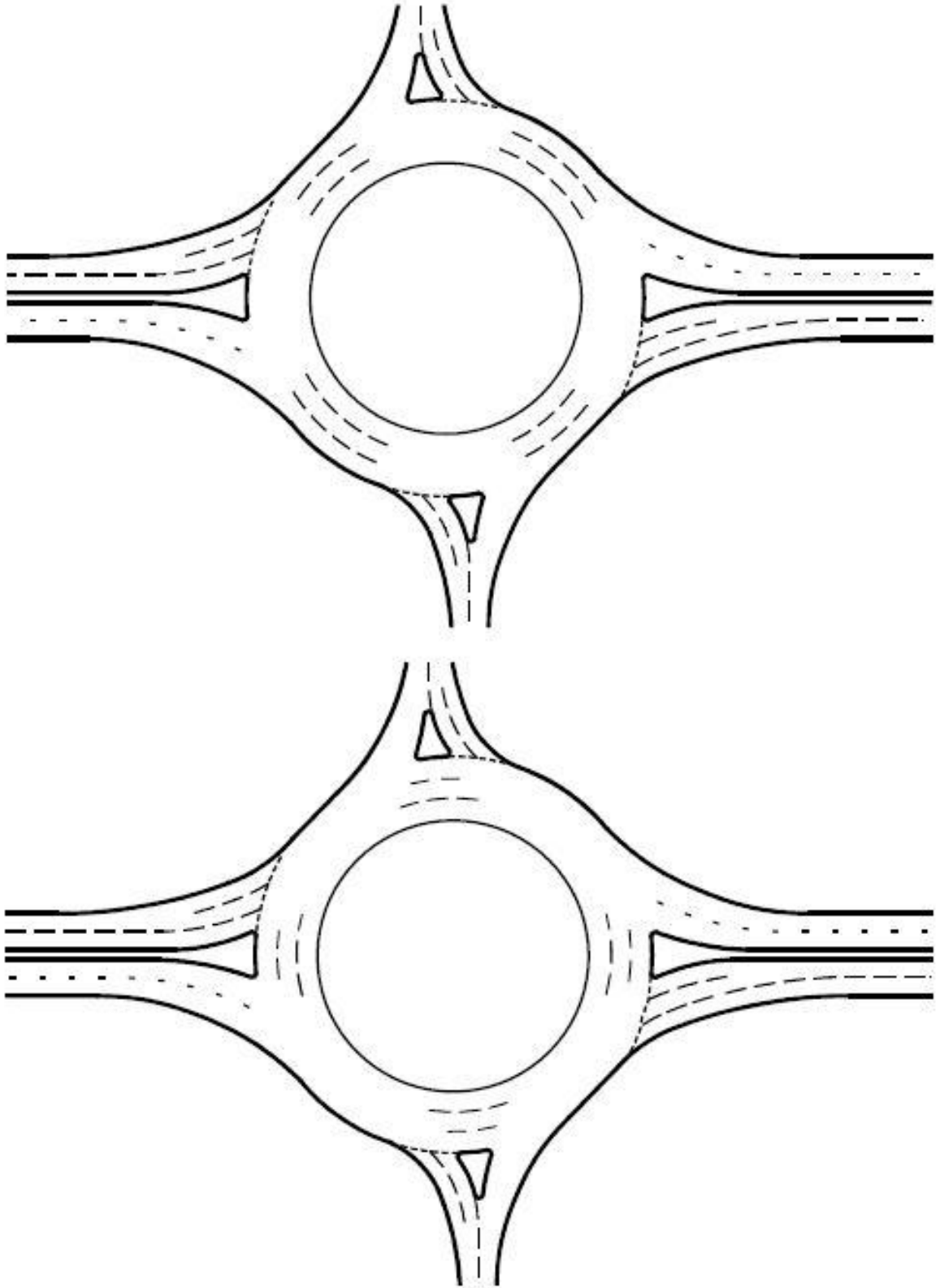
Figure D.4 Partial concentric markings
