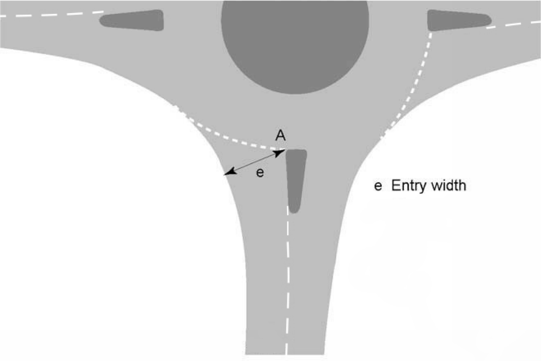
Figure 3.11 Entry width and approach half width
