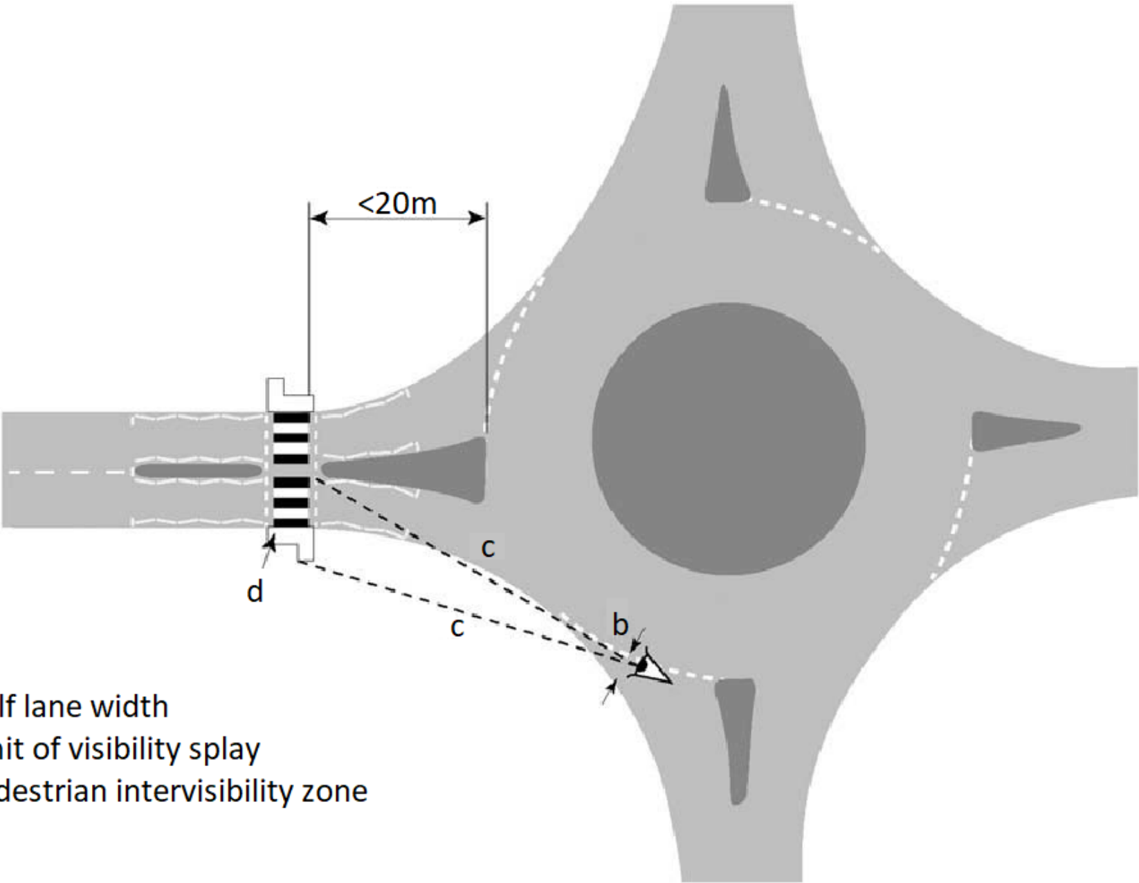
Figure 3.59 Visibility measured at entry to pedestrian crossing at next exit
