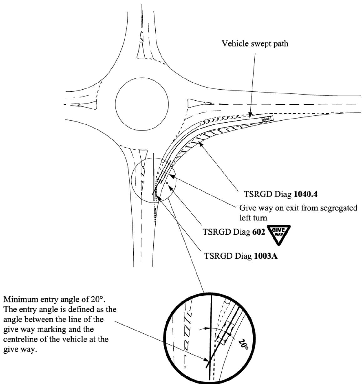
Figure 6.39 Physical SLTL with give way on exit
