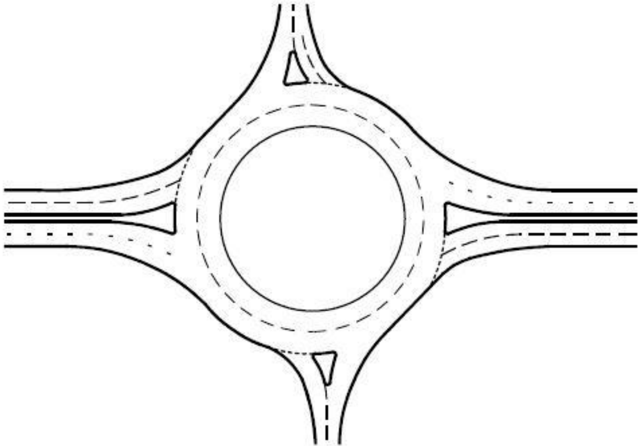
Figure D.3 Concentric markings
