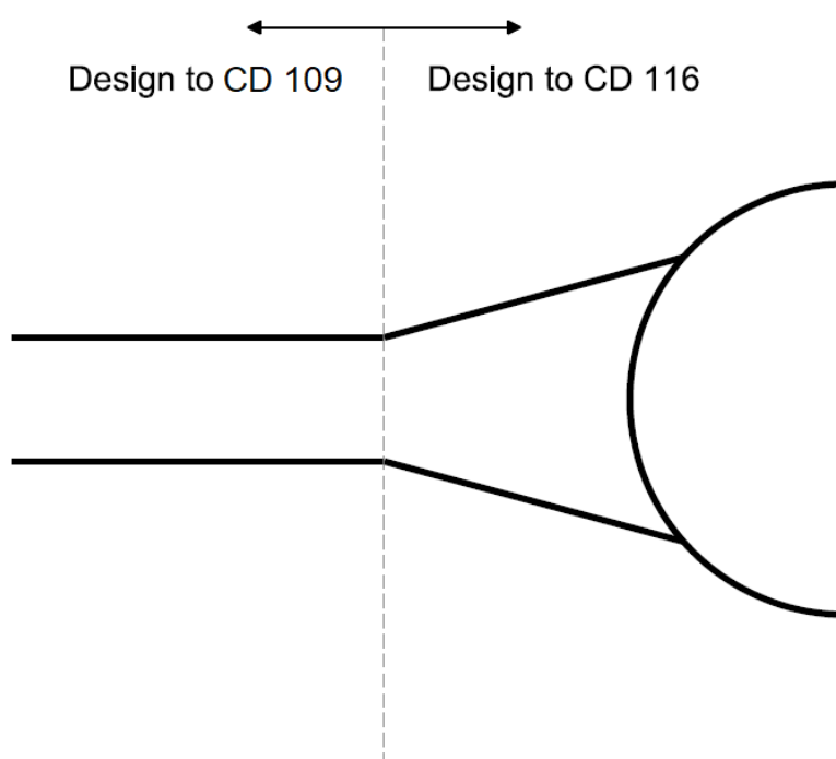
Figure 1.2 Scope of roundabout CD 116
