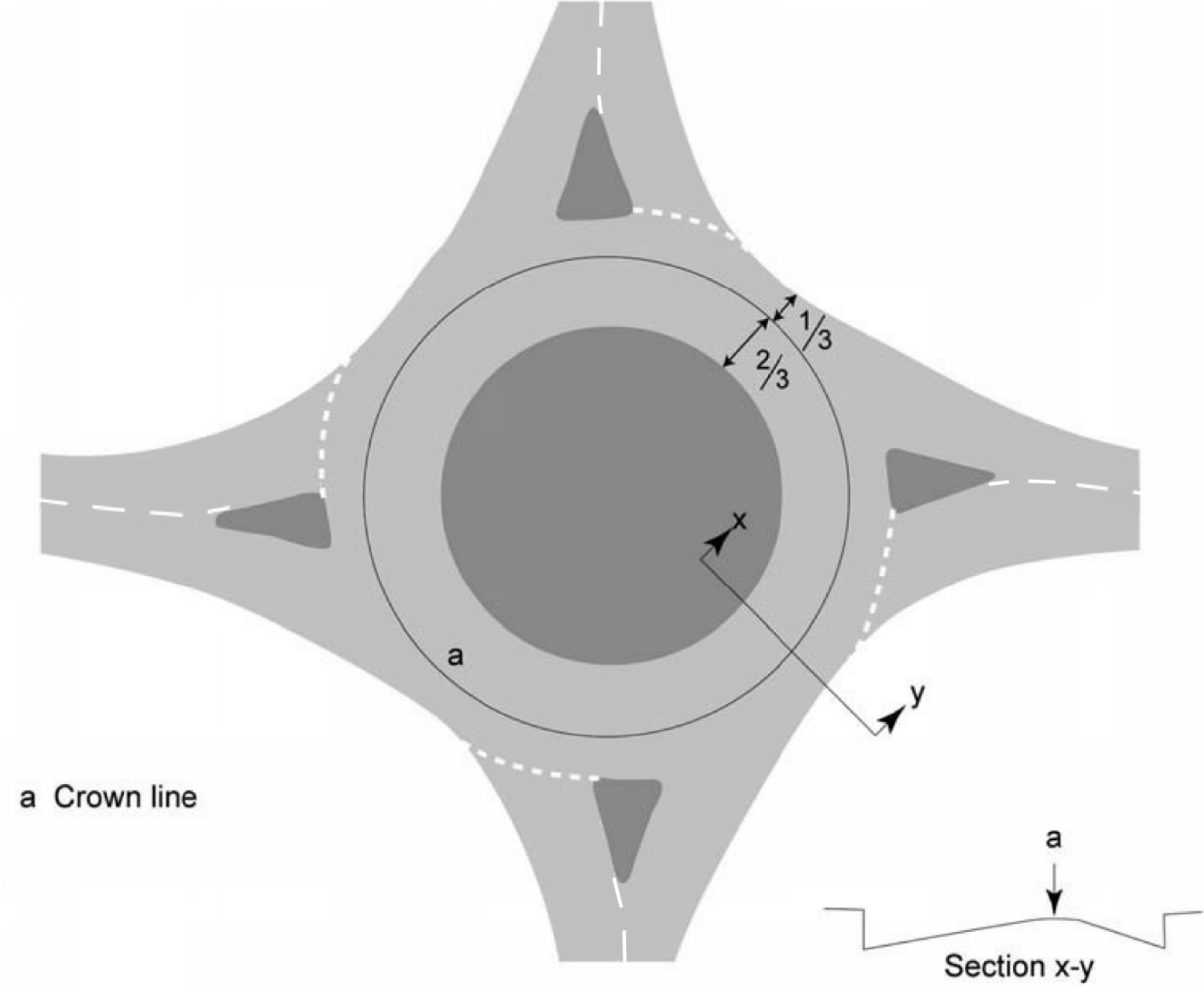
Figure 3.40.3N1b Using one crown line to divide the carriageway into the ratio 2:1
