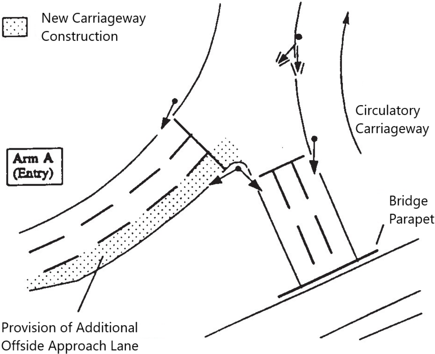
Figure 4.3.1N Provision of an additional offside approach lane
