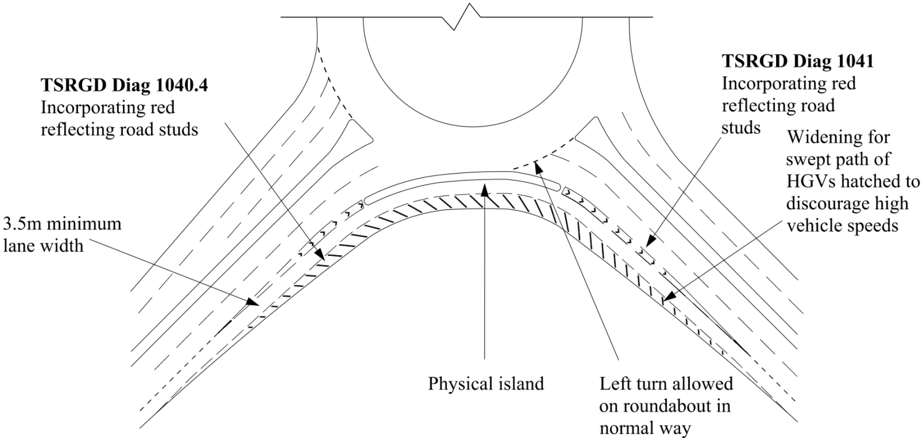
Figure 6.2.1 Generic physical SLTL
