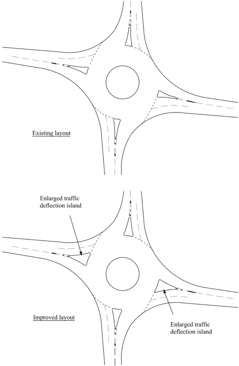
Figure 7.2N3a Example showing how traffic deflection island design can increase entry deflection at an existing roundabout
