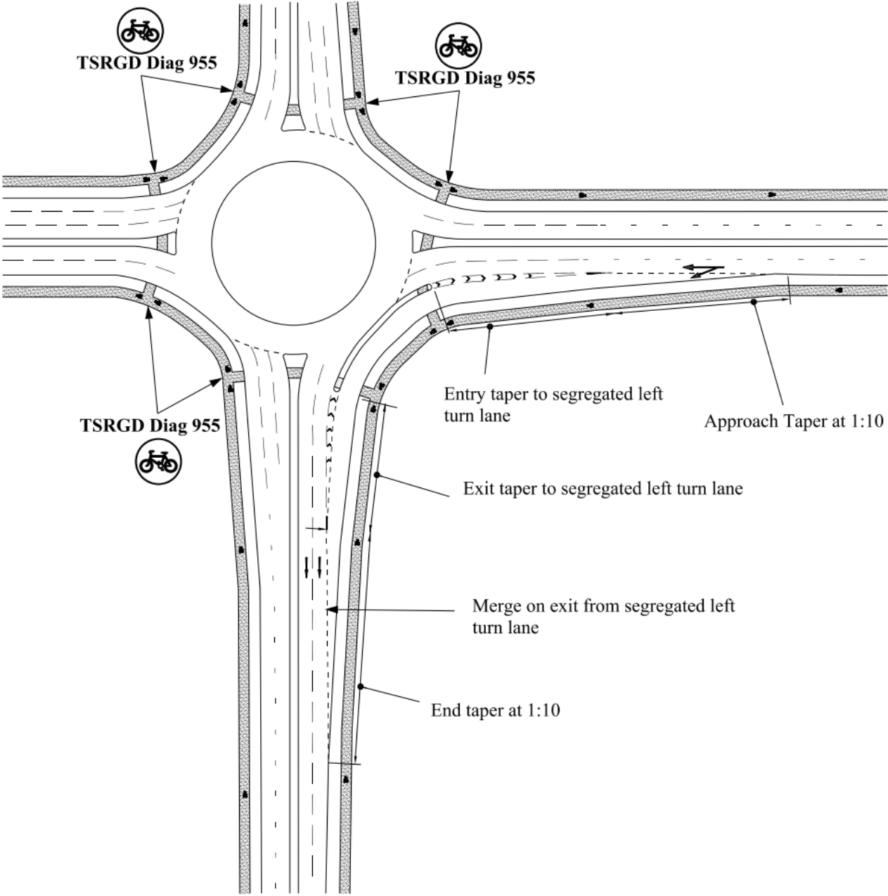
Figure 8.11N2a Diverge/merge layout SLTL island, 50 metres in length including cycle track
