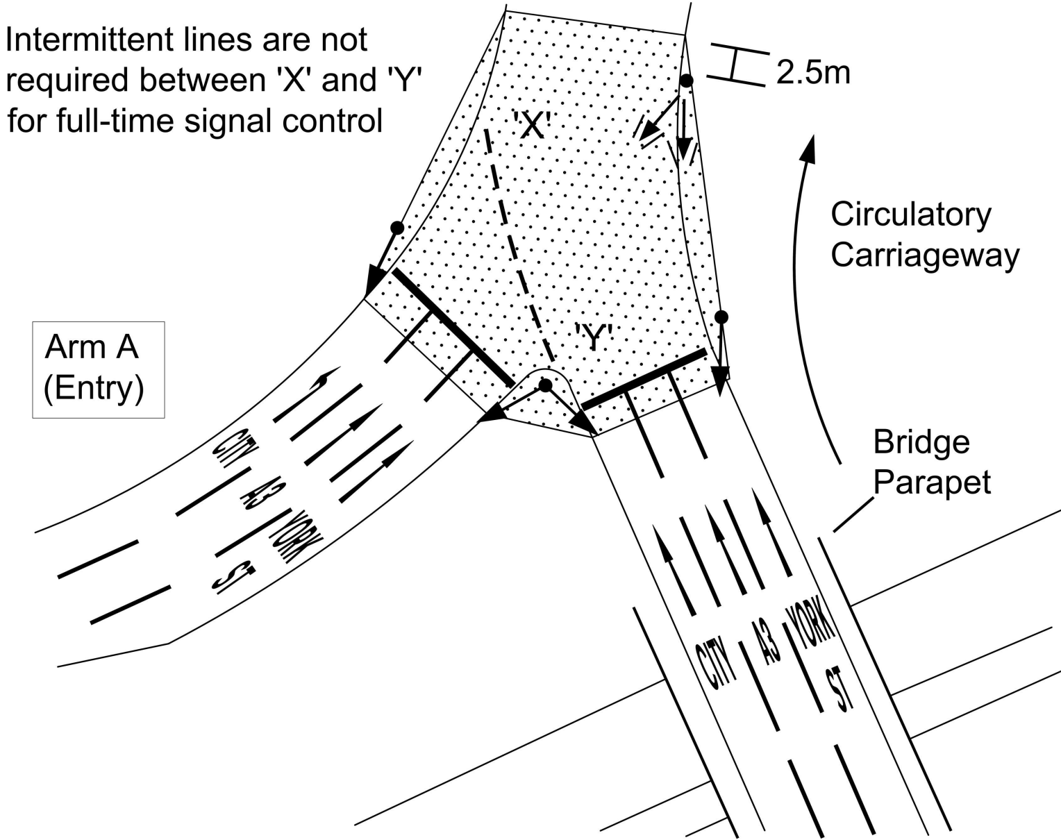
Figure 4.9.1 Junction intervisibility zone on a signal-controlled roundabout
