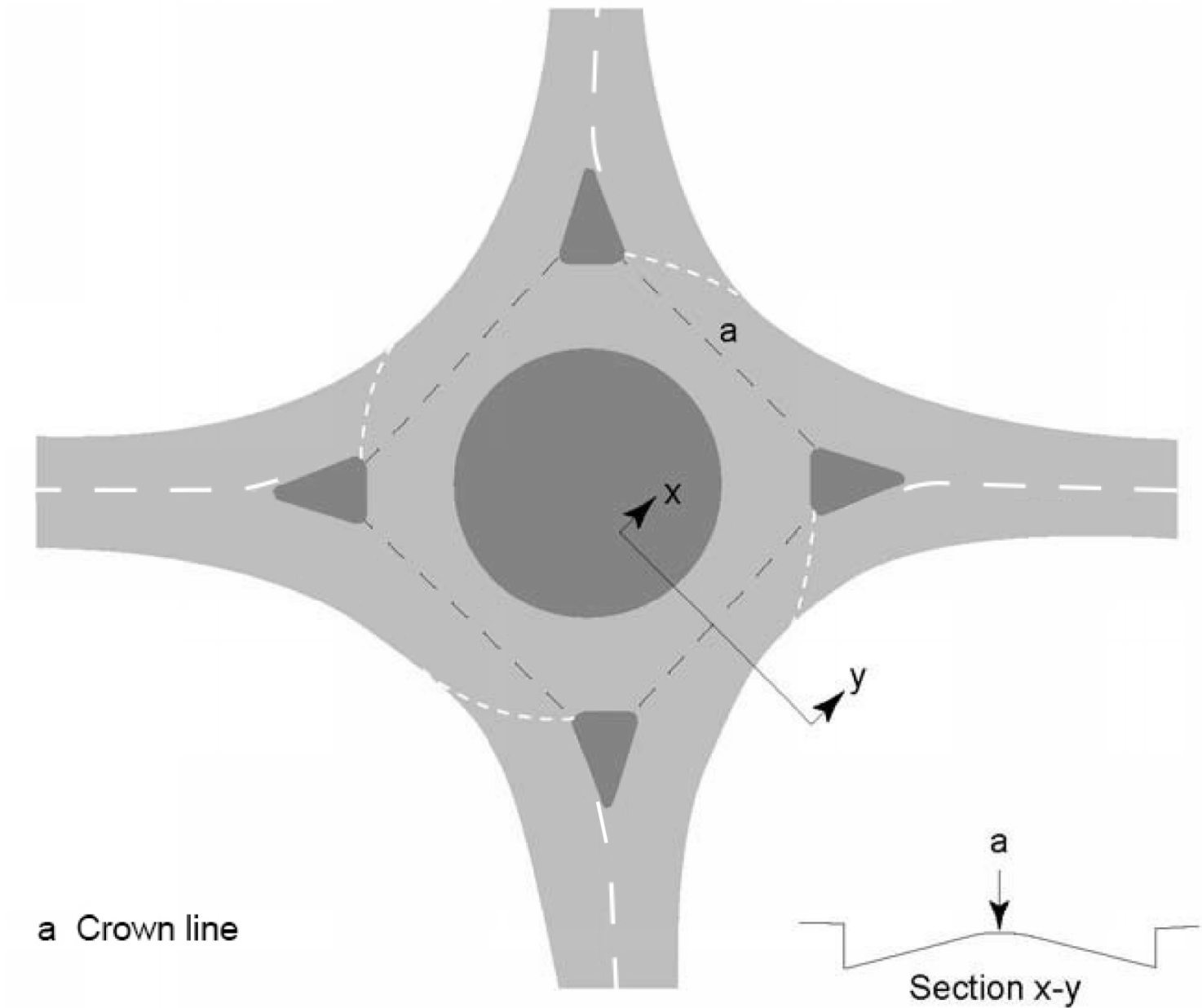
Figure 3.40.3N1a Using one crown line to join traffic islands
