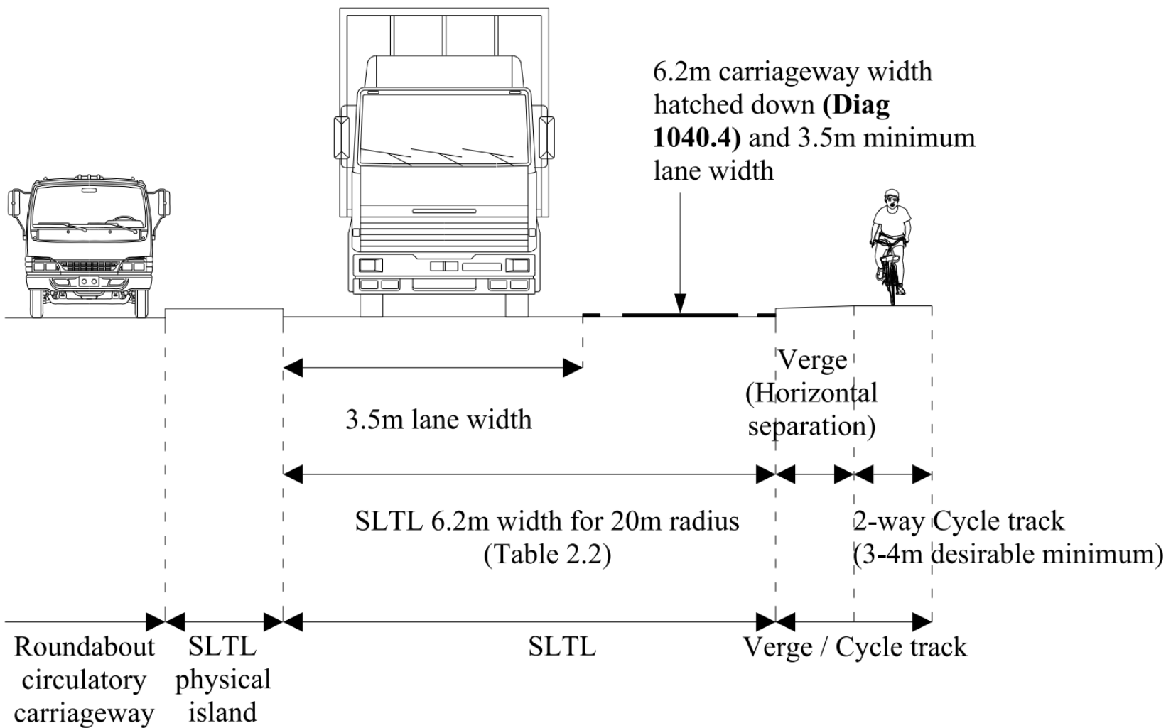
Figure 6.15 Indicative cross-section for SLTL island less than 50 metres in length with a radius of 20 metres (cross-section allowing for cycle traffic)
