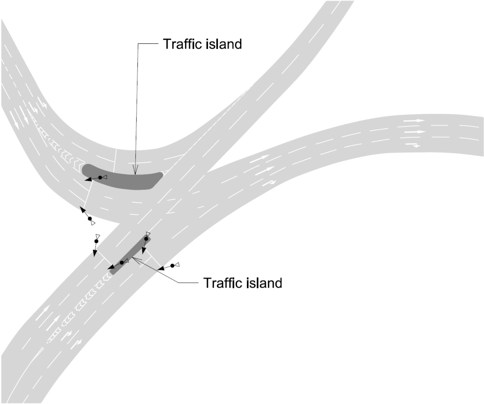
Figure 4.4 Indicative layout for a traffic island separating non-signal-controlled left-turn traffic from traffic entering the roundabout
