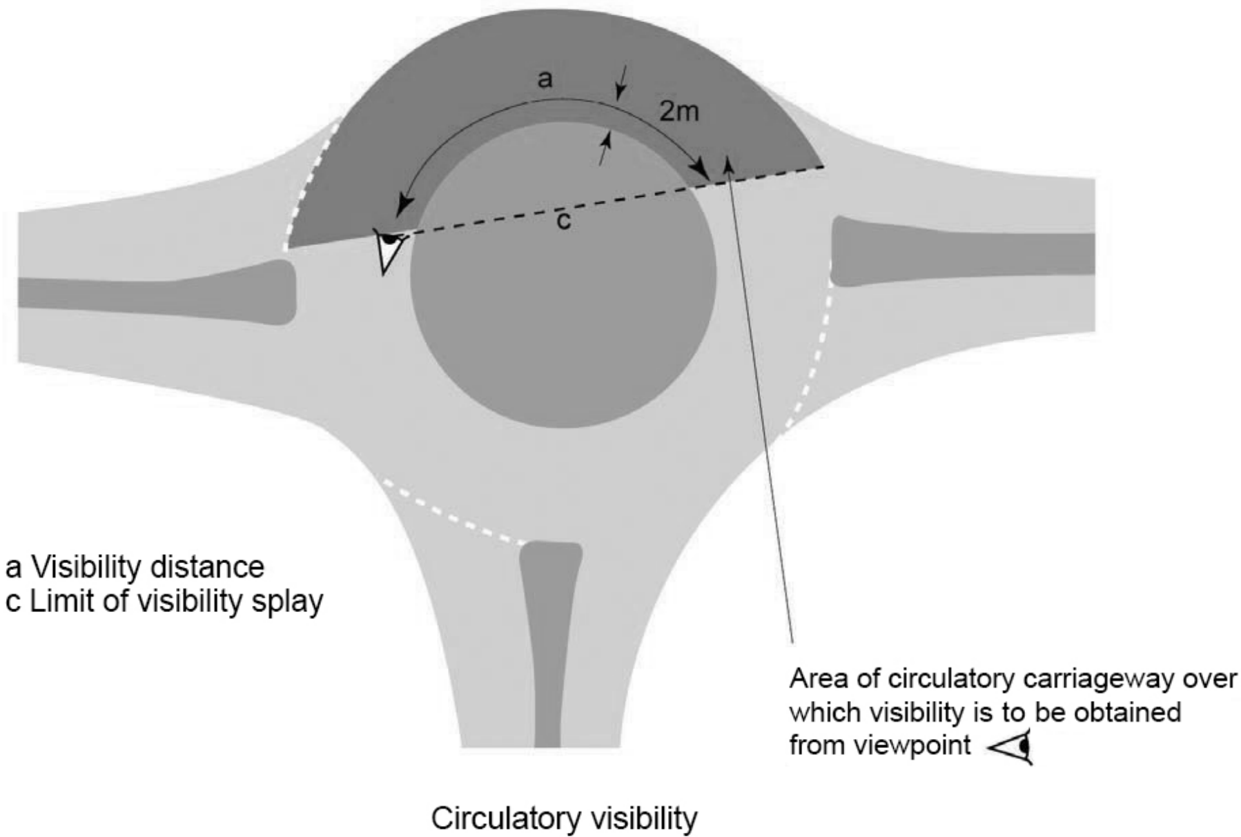
Figure 3.54 Circulatory visibility measurement for non-signal controlled and part-time signal-controlled roundabouts
