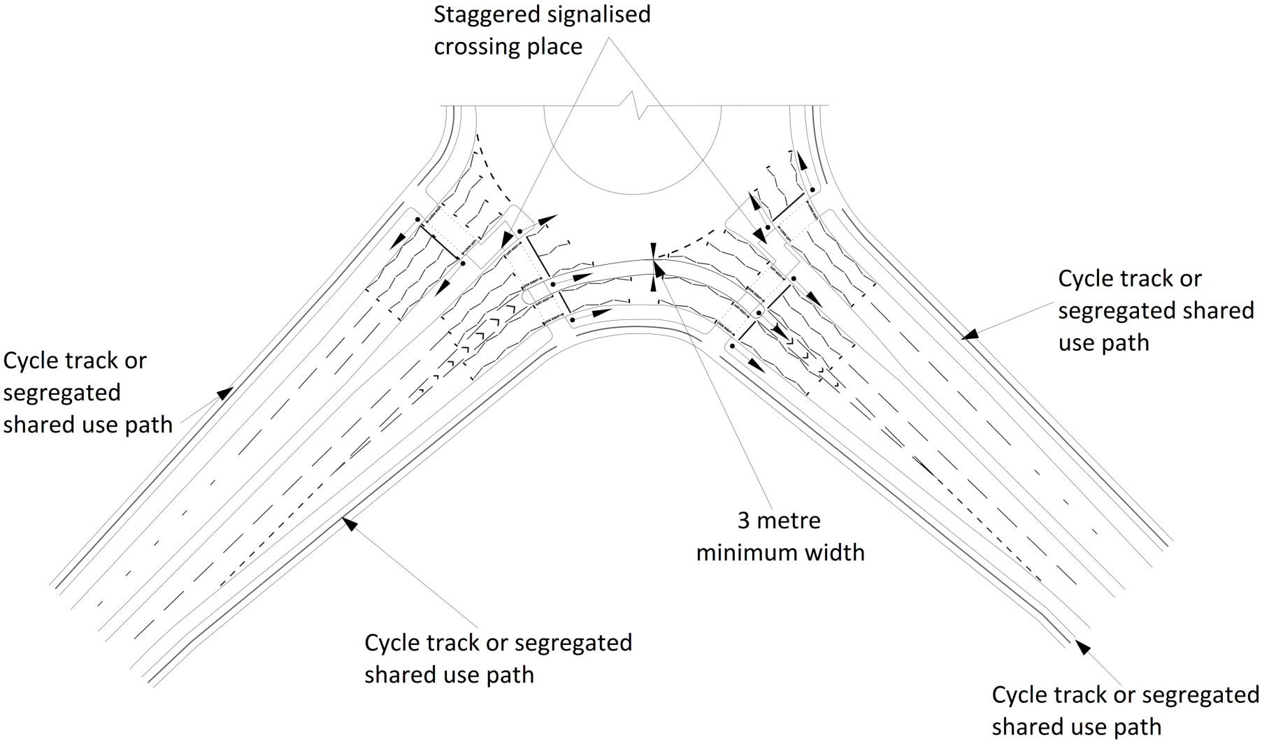
Figure 8.10 Cycle tracks and signal controlled crossing places at segregated left turn lane
