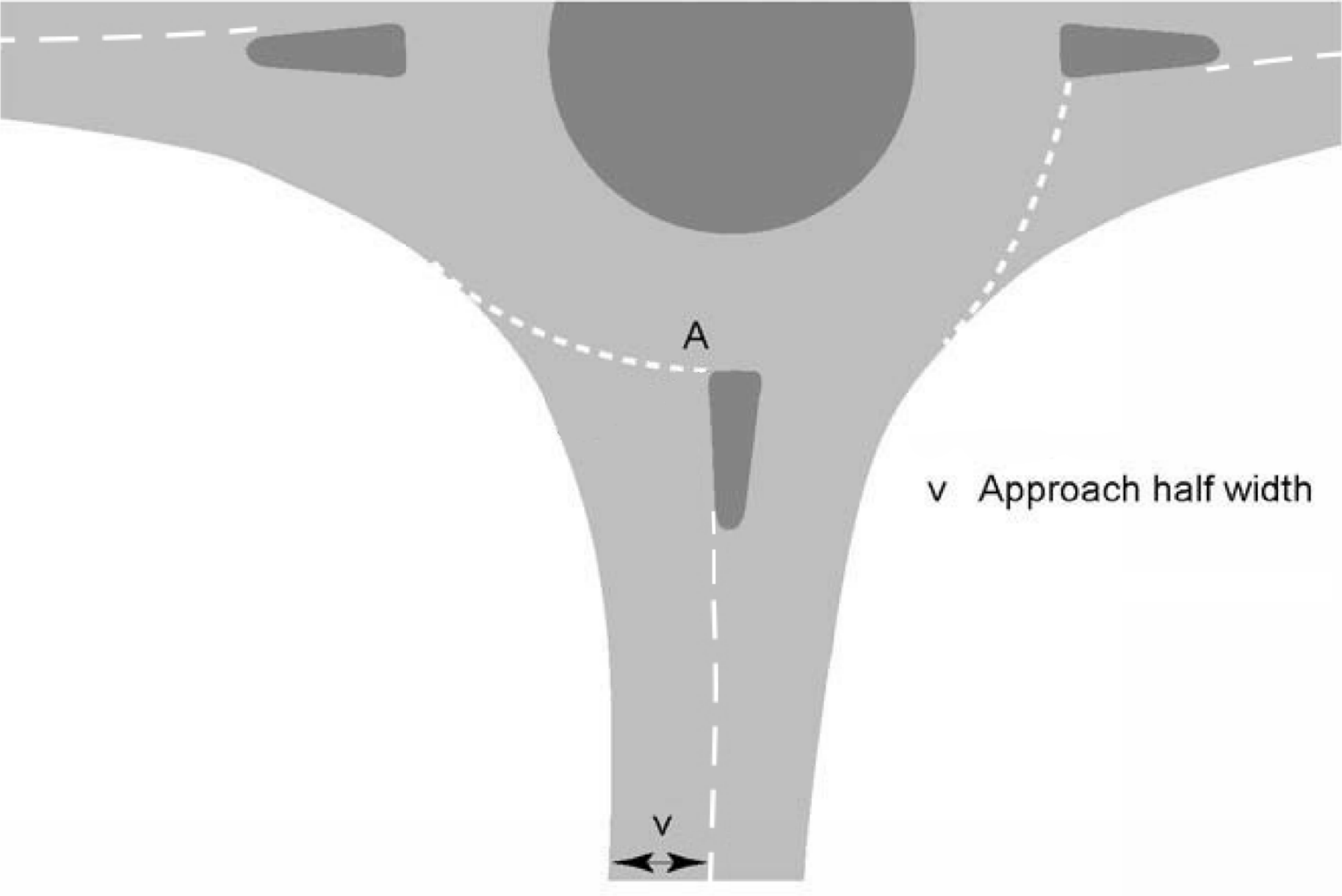
Figure 3.16 Entry width and approach half width
