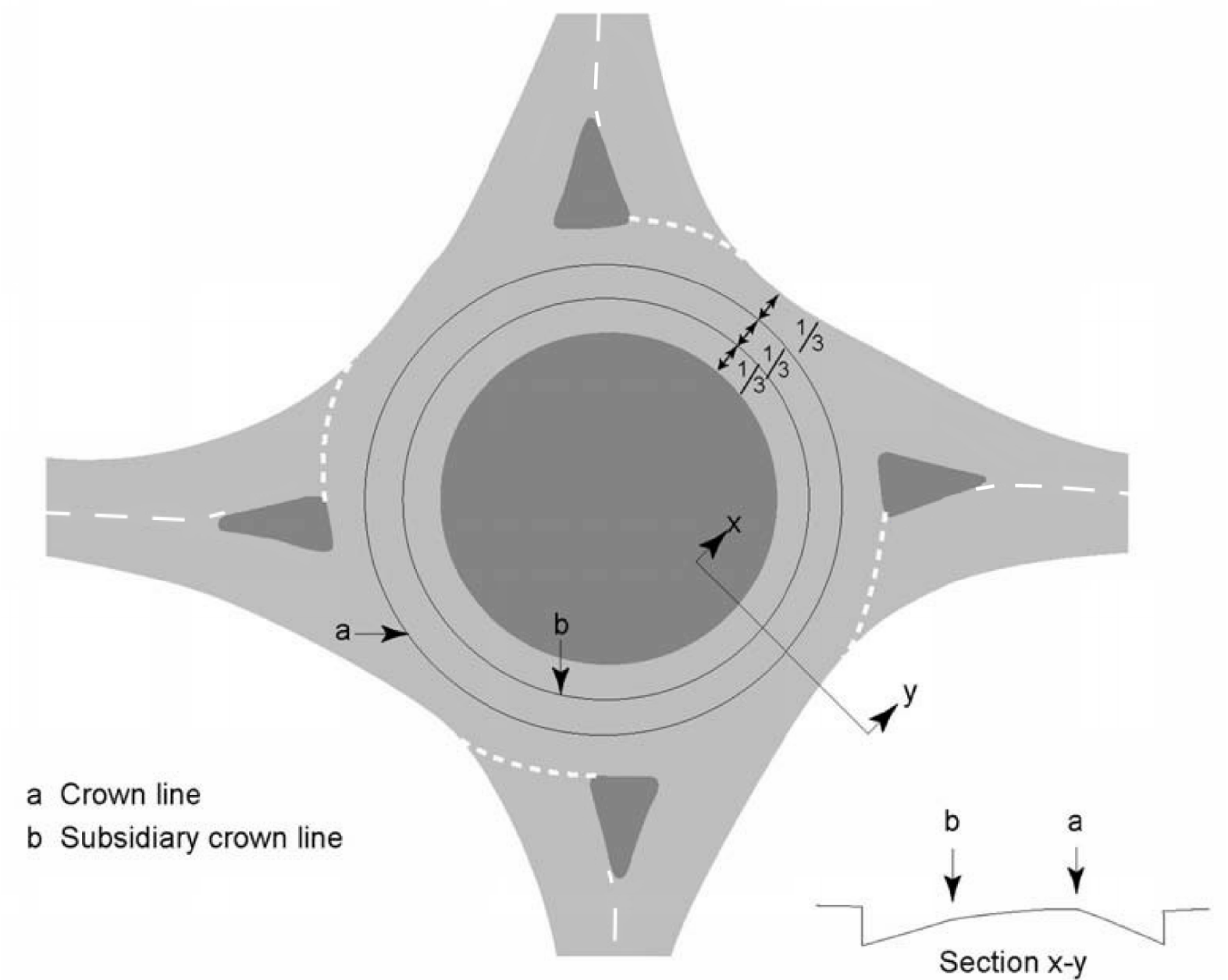
Figure 3.40.3N2 Using two crown lines
