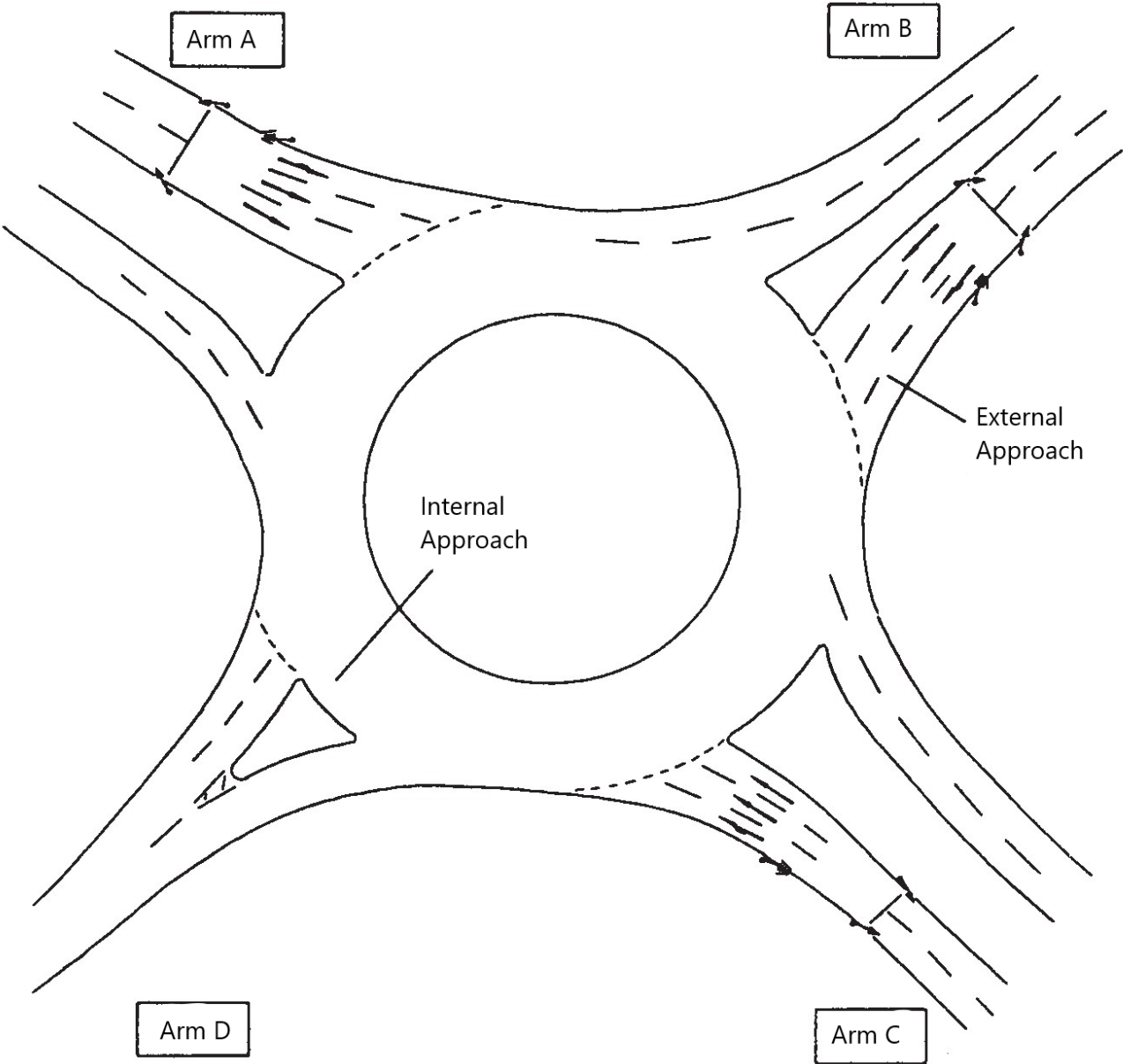
Figure 4.2.5 Signalised roundabout with indirect signal control
