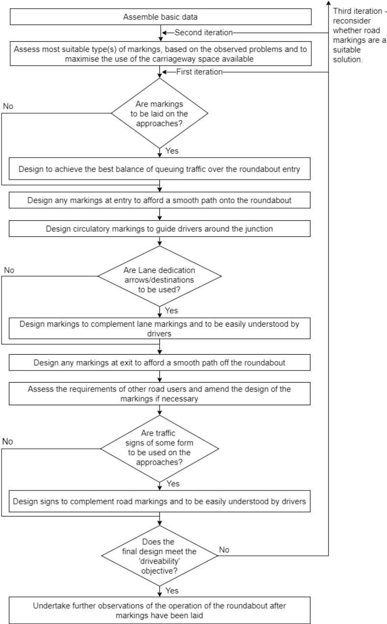
Figure D.2 Flow chart illustrating design principles
