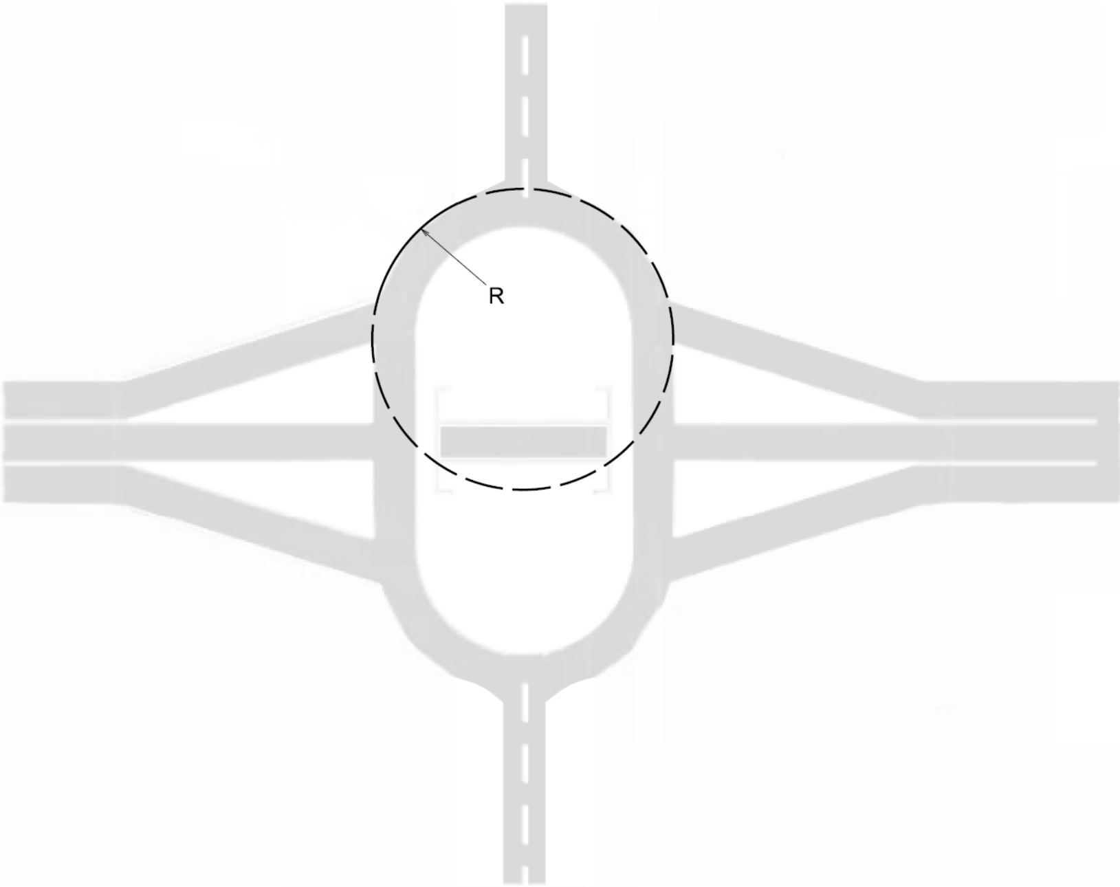
Figure 3.3 Inscribed circle diameter ( 2 \times R ) at a non-circular roundabout
