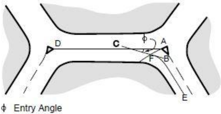
Figure B.1 Measurement of entry angle where the distance circulatory carriageway between an entry and the next exit is approximately straight and more than about 30 metres
