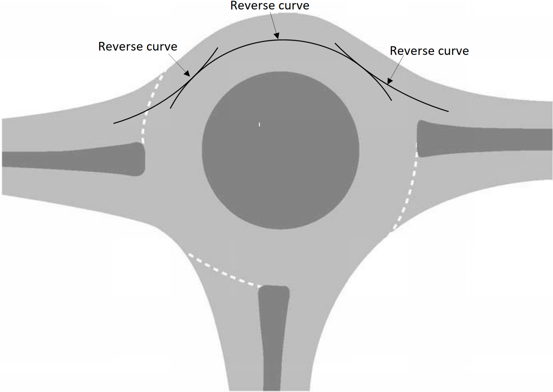
Figure 3.6.8N2 Three-arm roundabout illustrating reverse curvature
