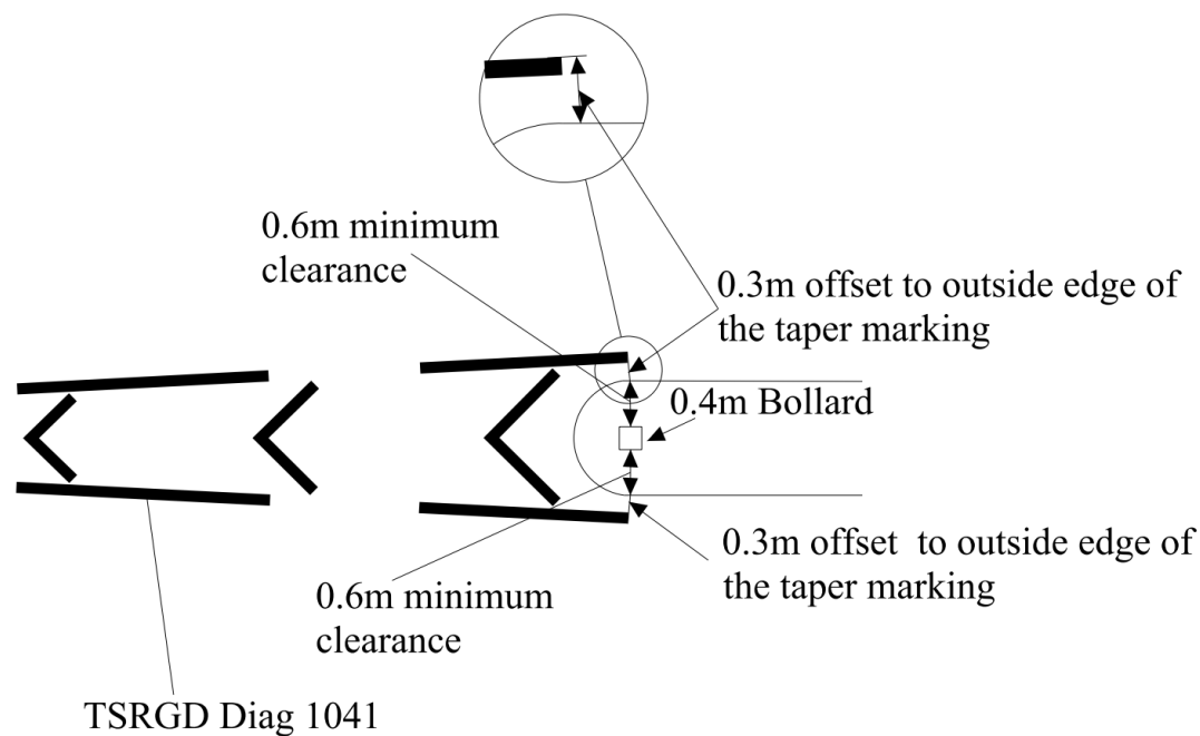
Figure 6.37.2 Termination of taper hatching at physical island
