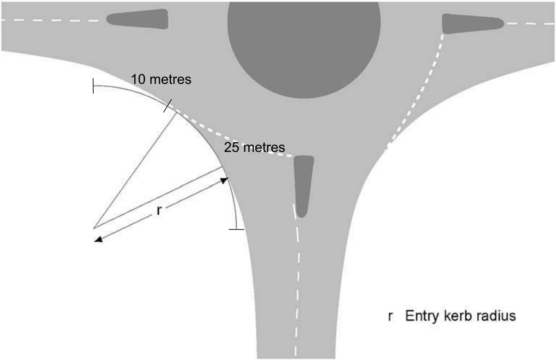
Figure 3.19 Entry kerb radius
