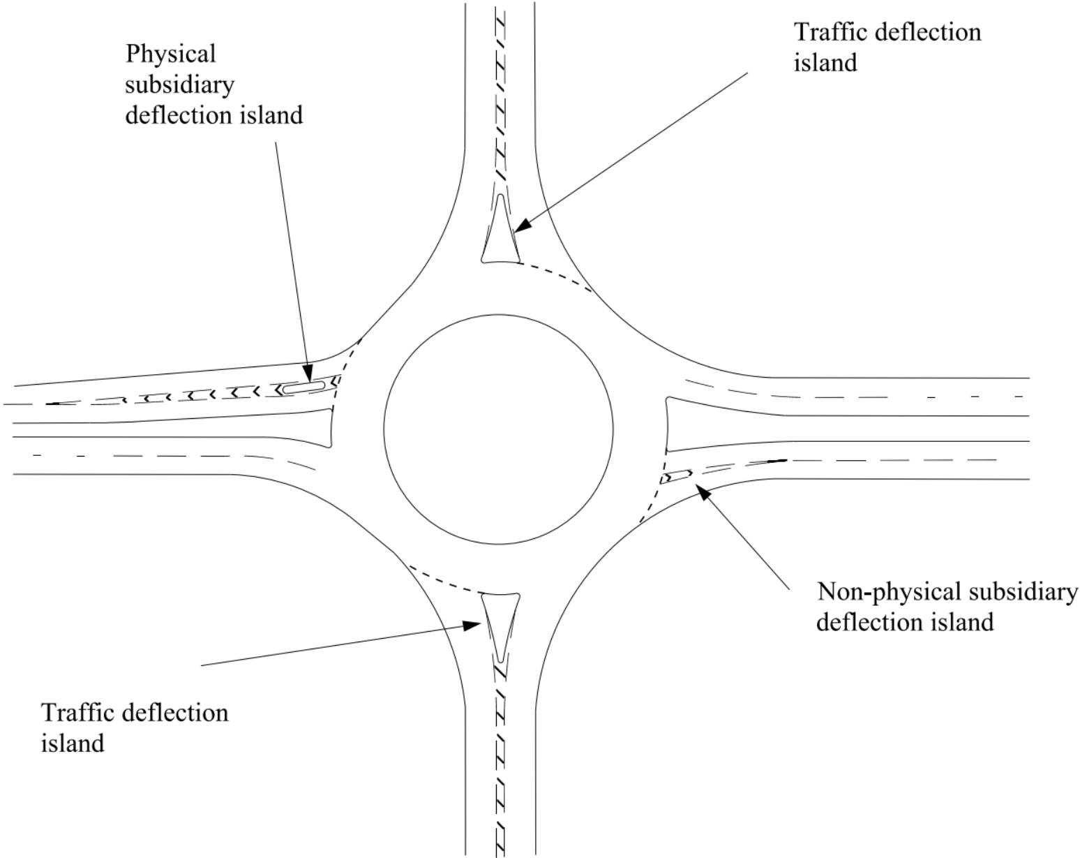
Figure 7.2N1 Example of traffic deflection islands and physical and non-physical SDIs (crossing facilities not shown to aid clarity)
