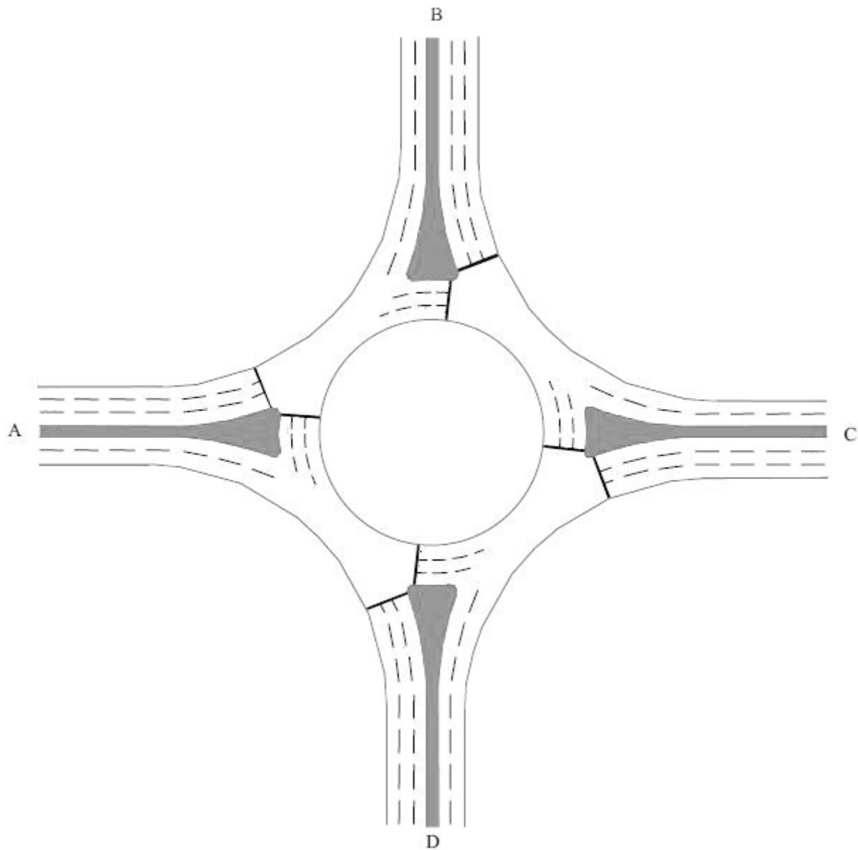
Figure 2.7 Illustrative layout of a signal-controlled roundabout
