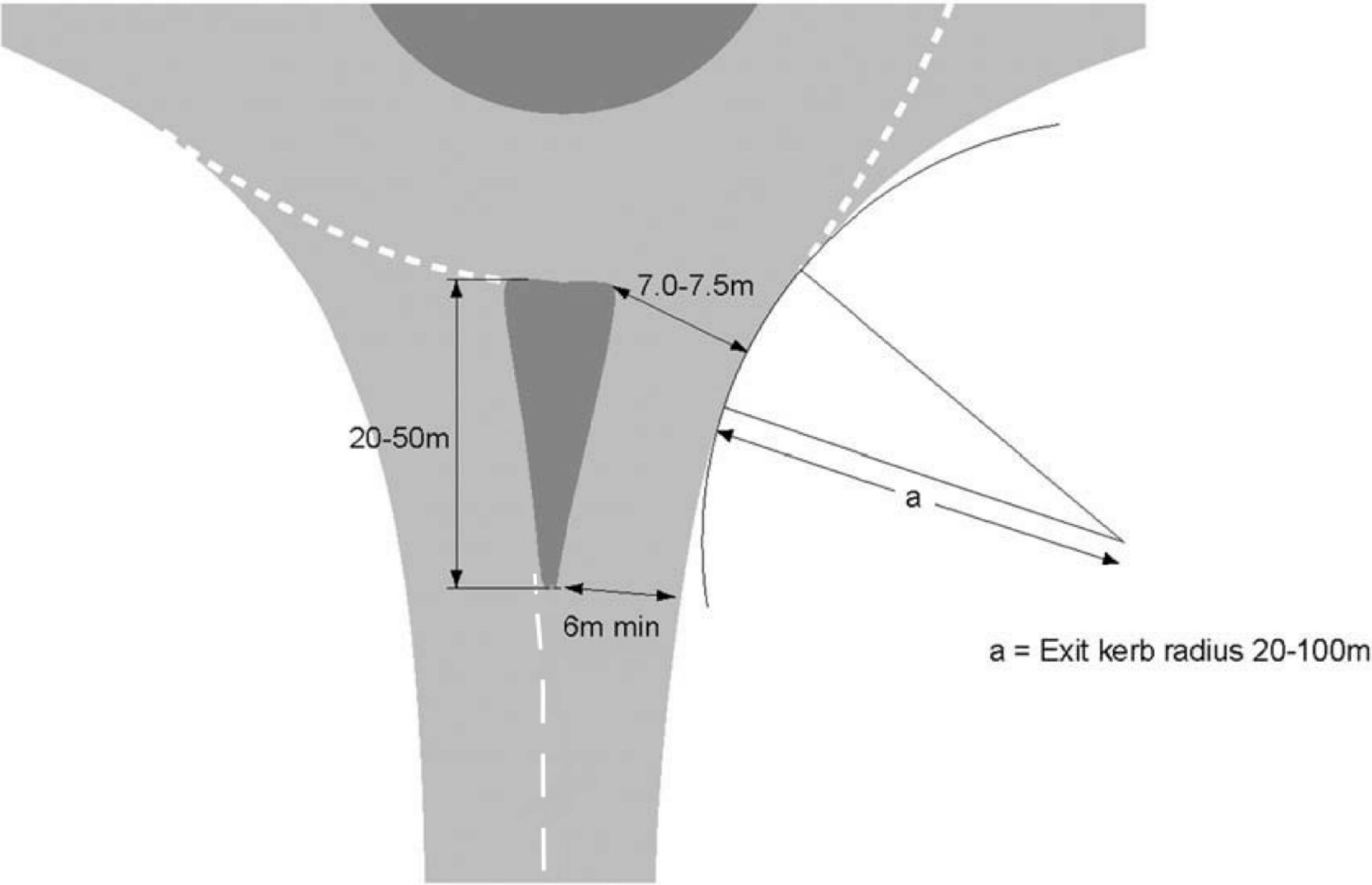
Figure 3.28 Typical single carriageway exit at a normal roundabout with a long traffic island
