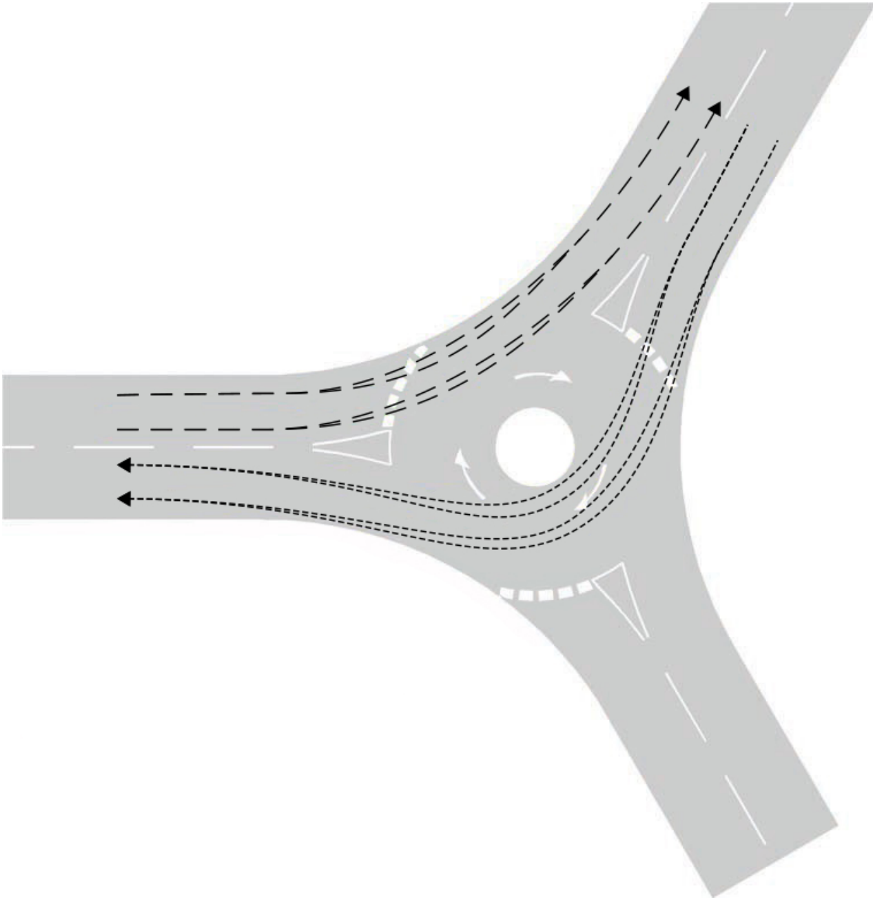
Figure 5.4Nb Determination of vehicle path and white circle location using swept paths (3-arm Y-junction)
