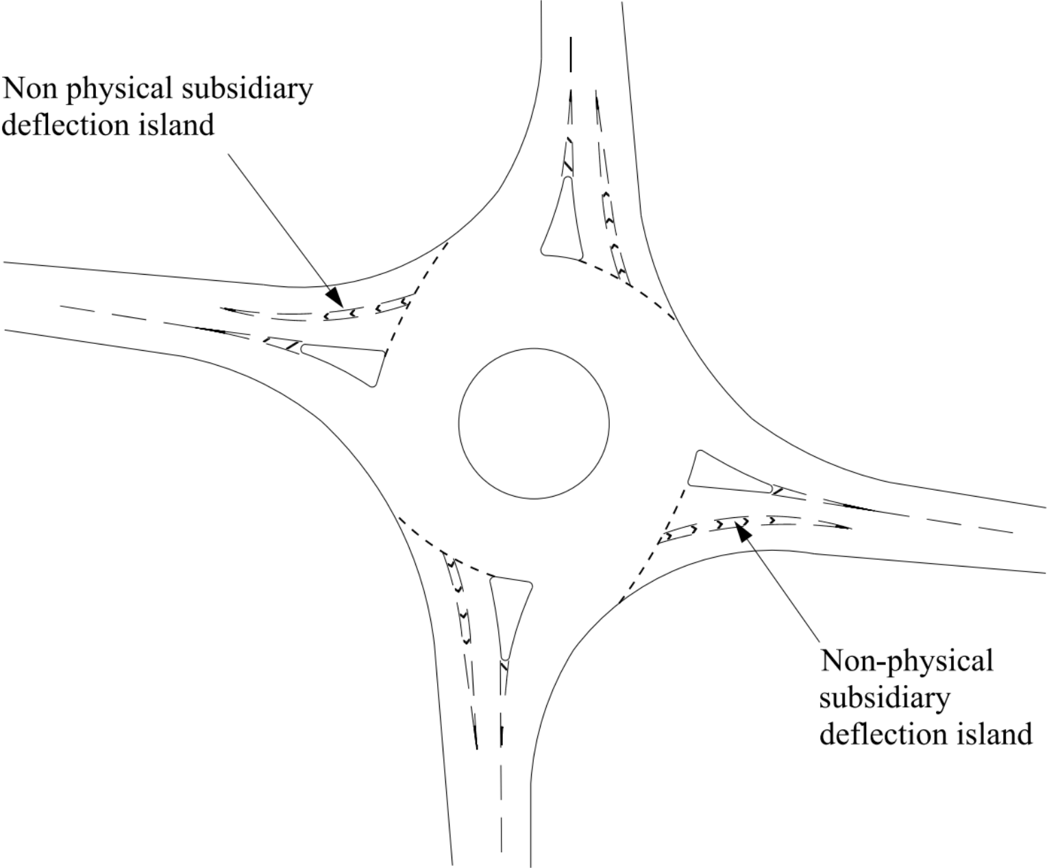
Figure 7.2N3b Example showing how a non-physical SDI can increase entry deflection at an existing roundabout
