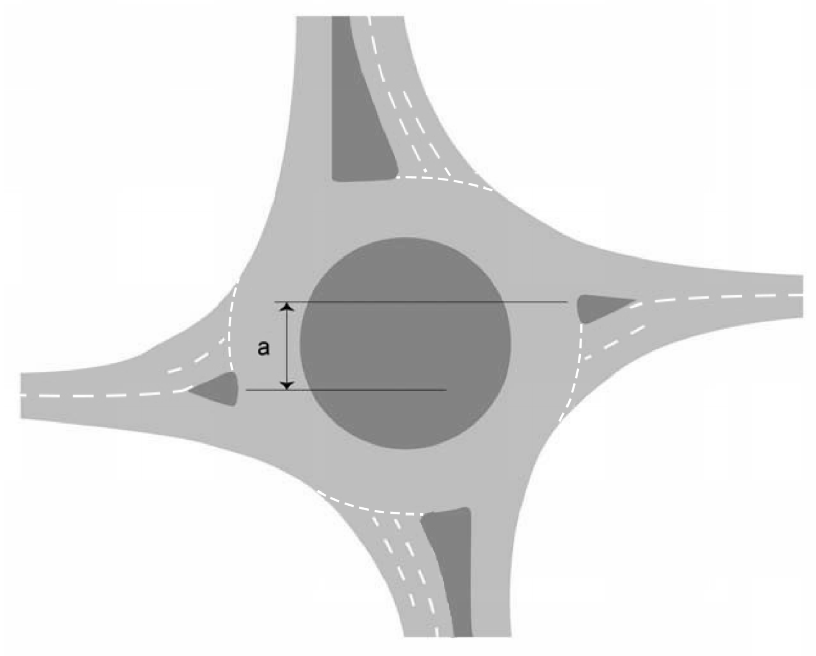
Figure 3.26.1 Staggering of east-west arms to increase deflection
