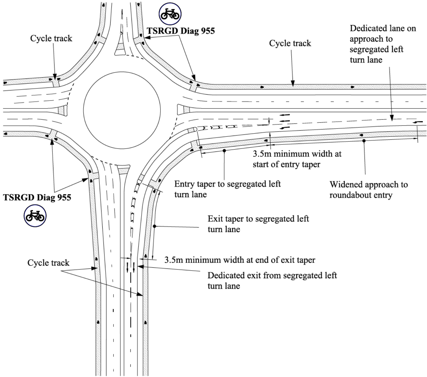
Figure 8.11N2b Dedicated approach and exit for SLTL including cycle track
