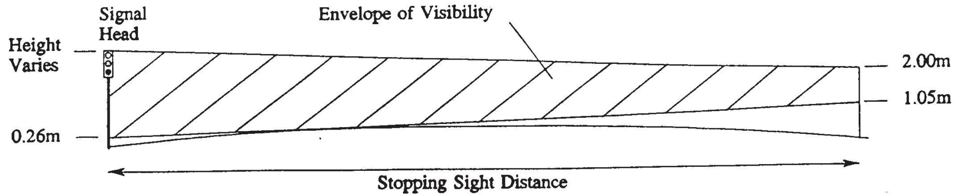
Figure 4.8 Visibility requirements to a signal head
