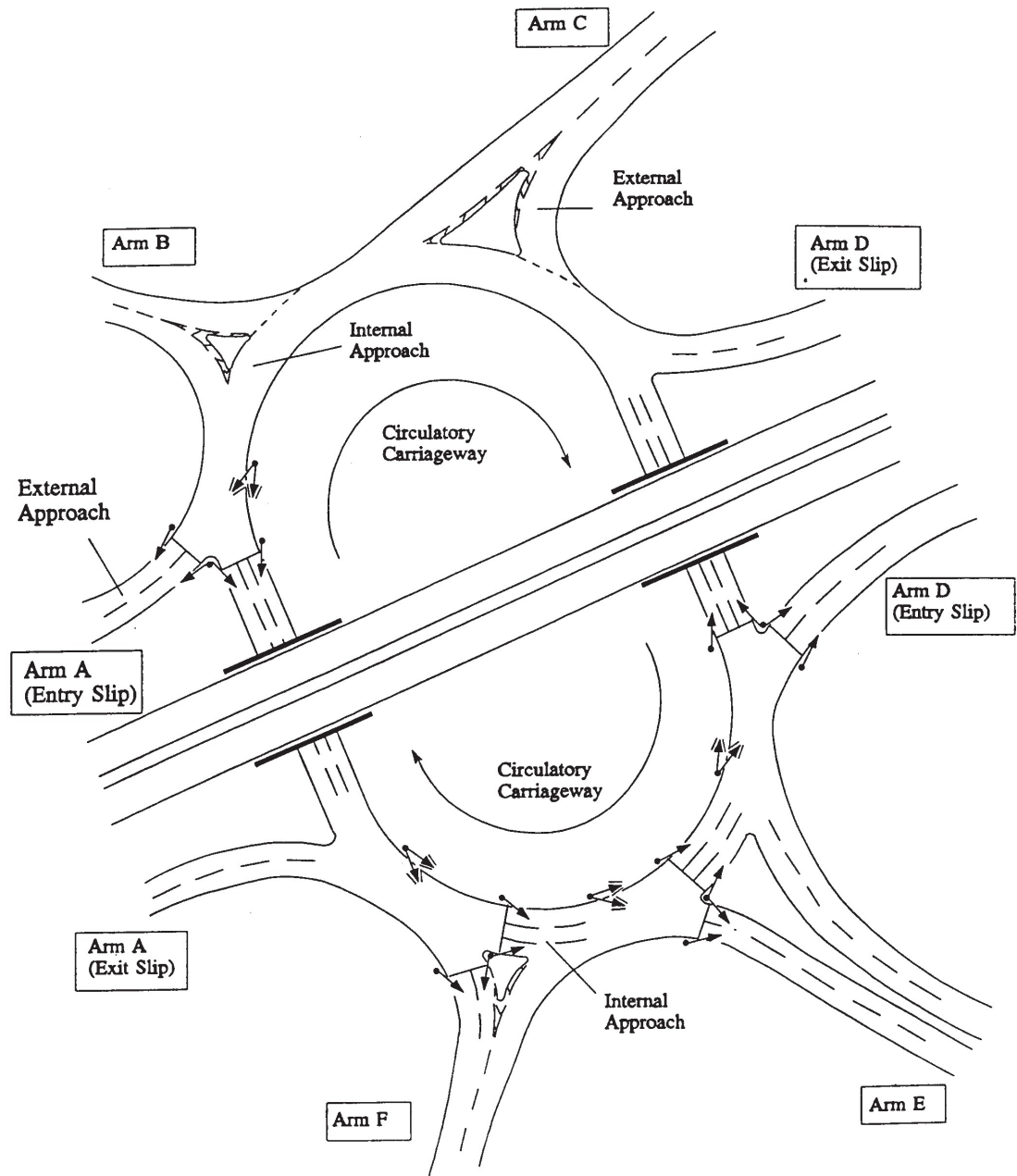
Figure 4.2.1 Example of a large signalised roundabout with partial, direct signal-control
