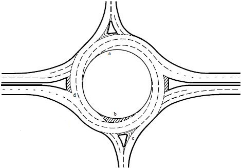
Figure D.6 Spiral markings
