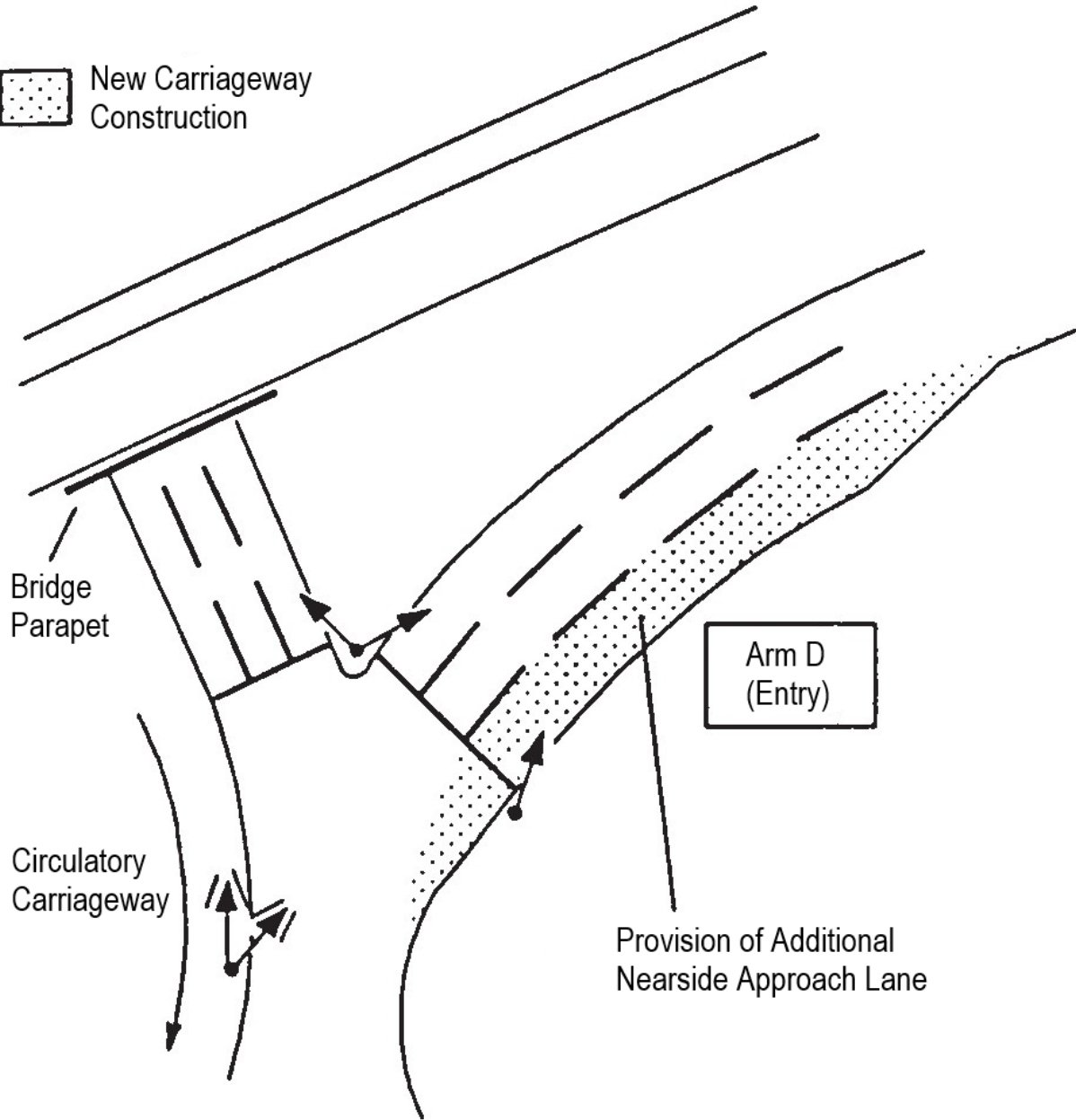
Figure 4.3.2N1 Provision of an additional nearside approach lane
