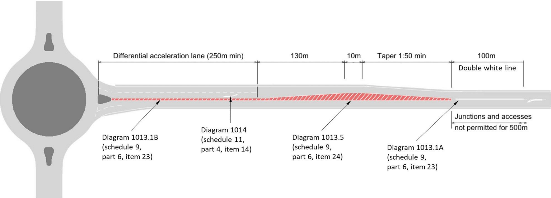
Figure 3.31 Layout of differential acceleration lane
