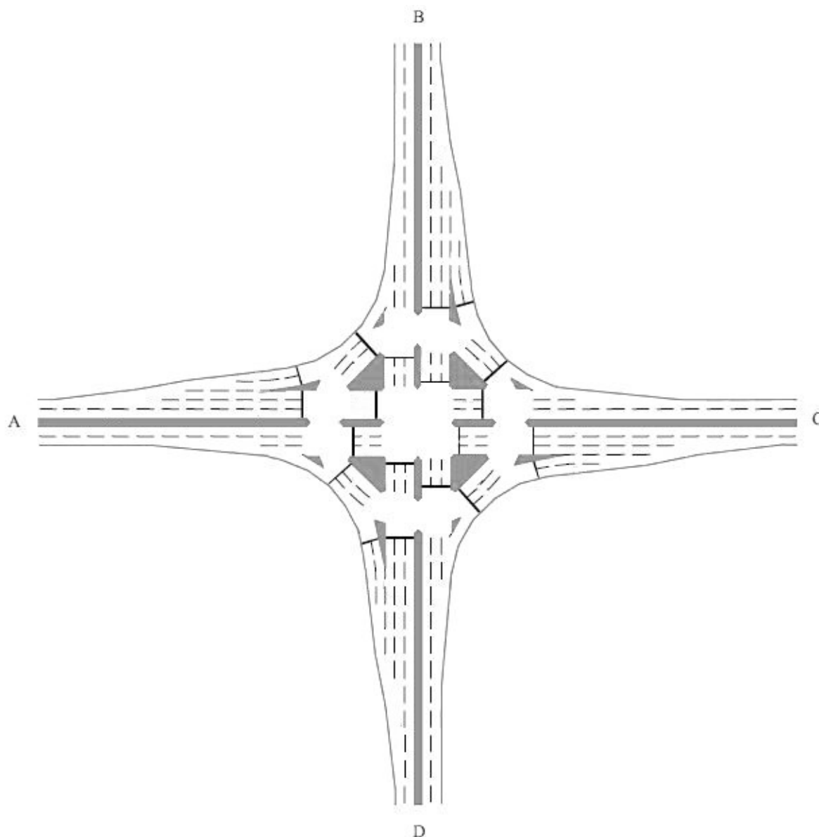
Figure 2.8b Illustrative layout of a double-through-about
