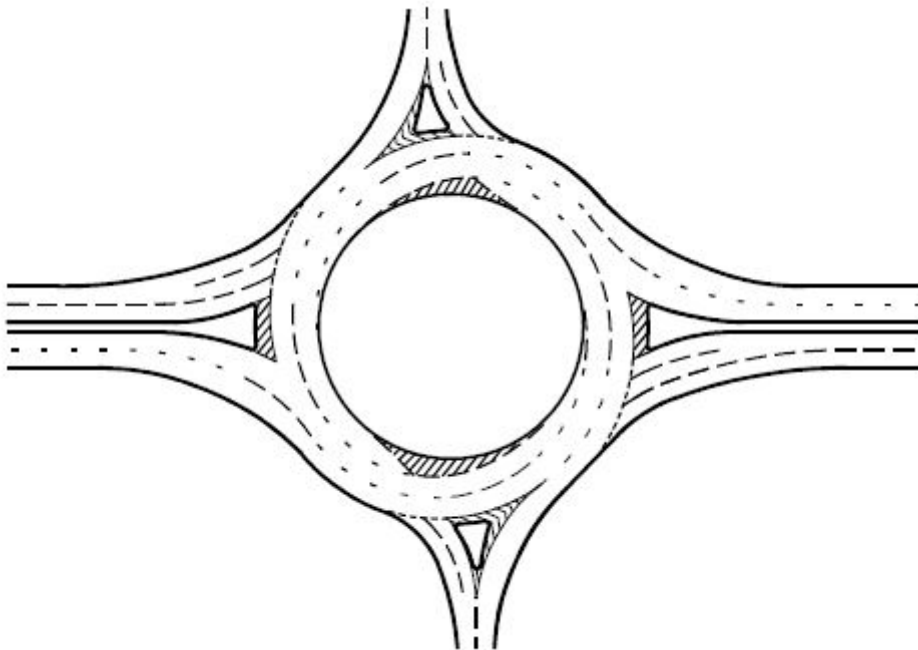
Figure D.7 Use of different lane types within a spiral markings system
