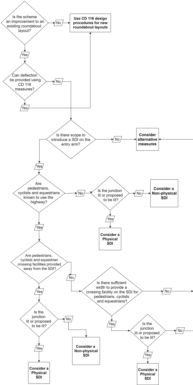
Figure C.2 Example of flow chart decision process for incorporation of SDI
