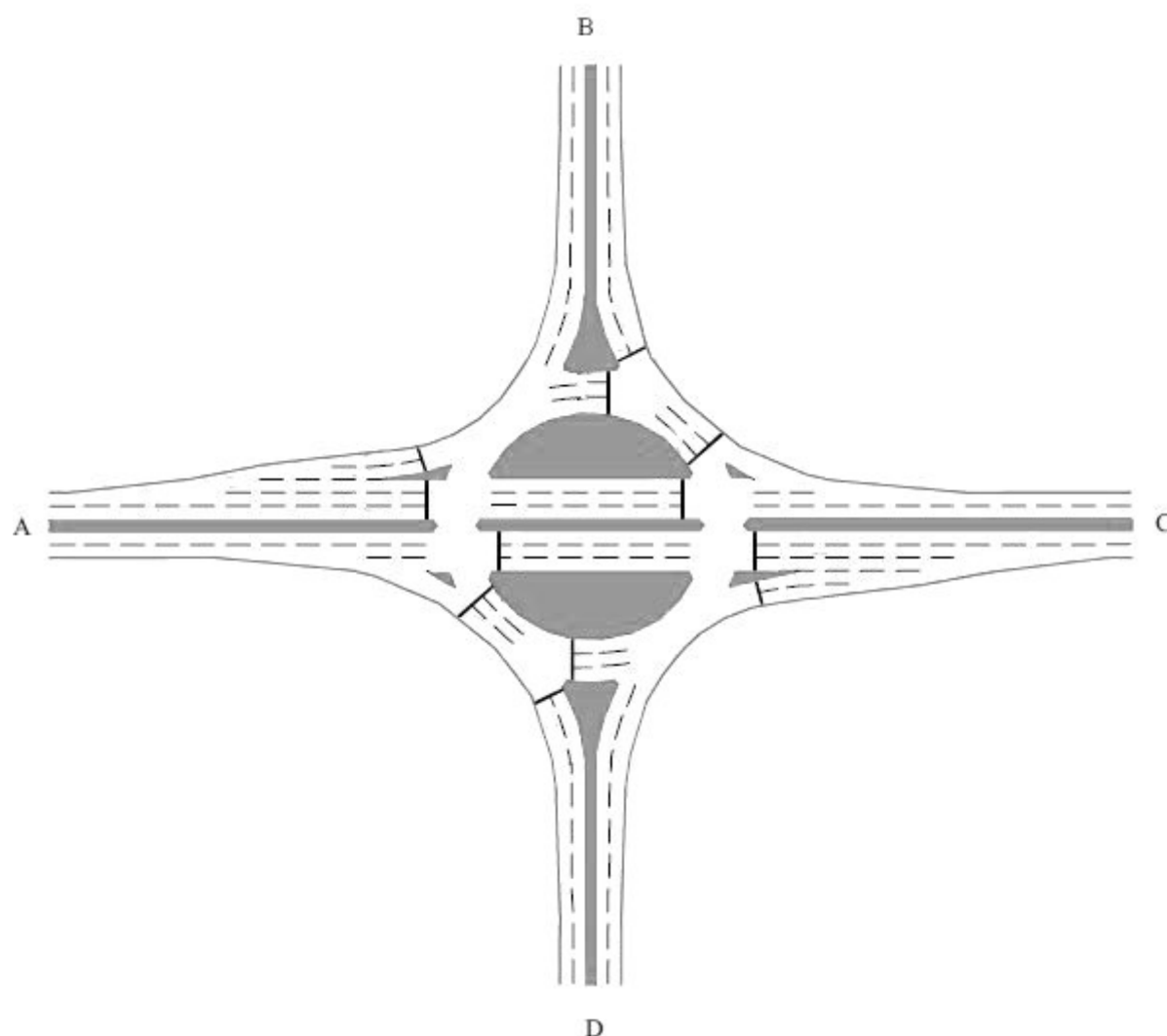
Figure 2.8a Illustrative layout of a through-about
