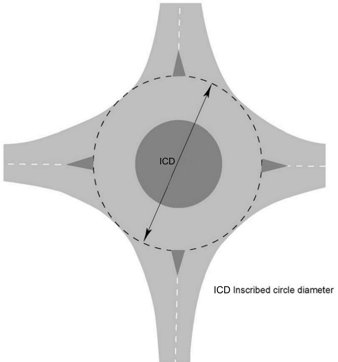
Figure 3.2 Inscribed circle diameter at a normal or compact roundabout
