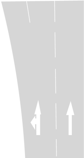
Figure 3.27.6b Example of entry markings
