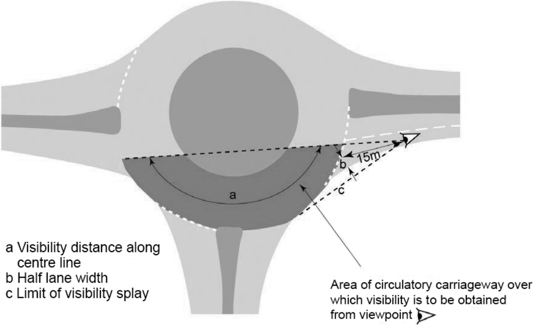
Figure 3.49N Forward visibility measured at entry
