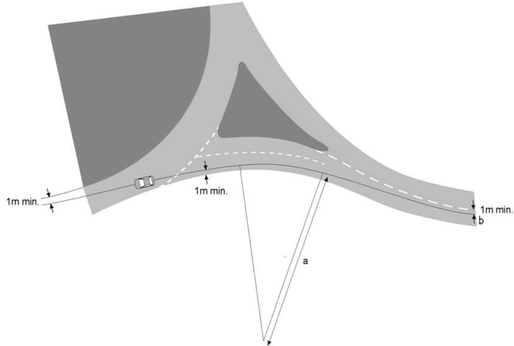
Figure 3.23 Determination of entry path radius for the left turn where the approach curves to the right
