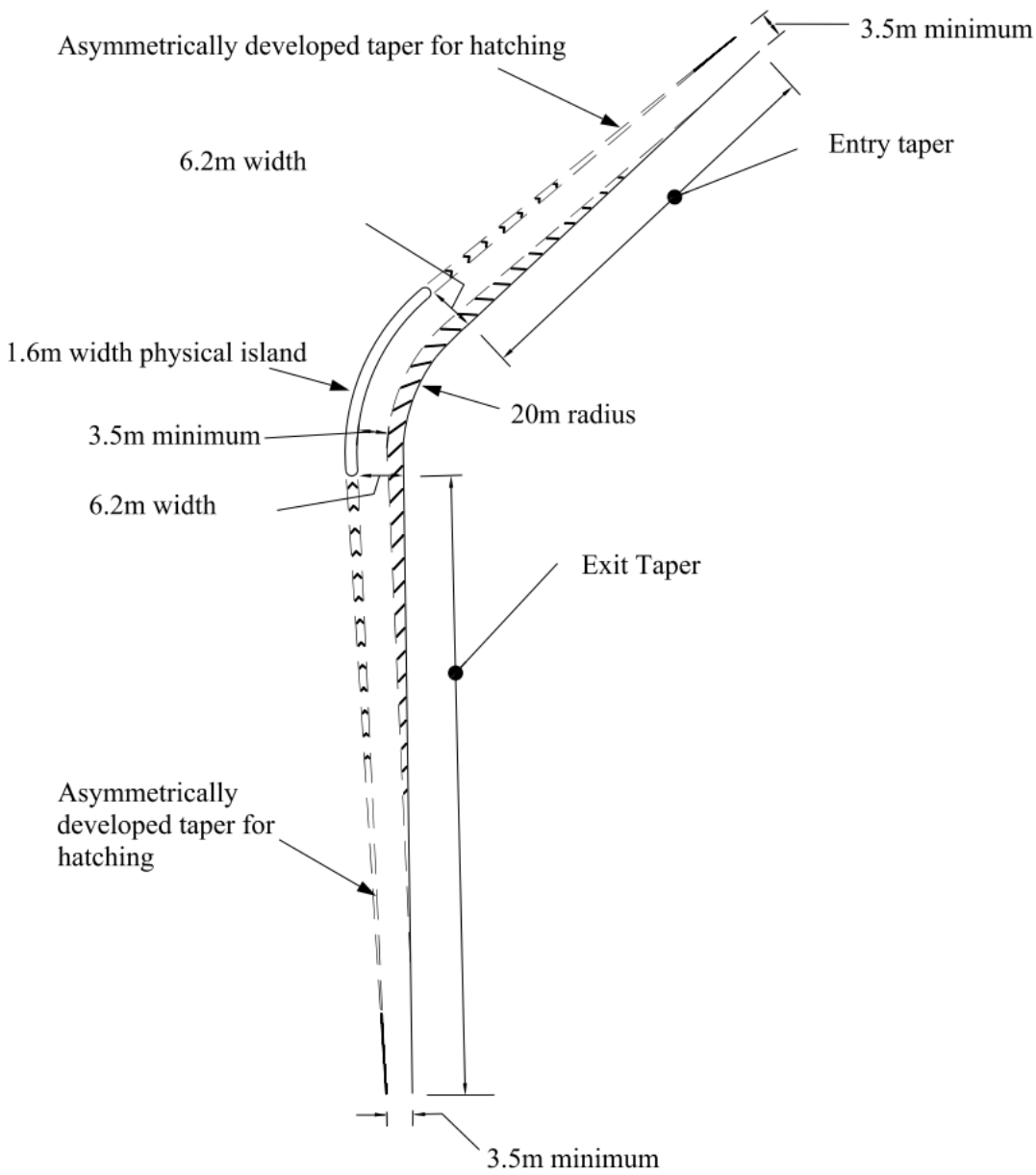
Figure 6.37.1 Example of calculation of entry/exit taper length
