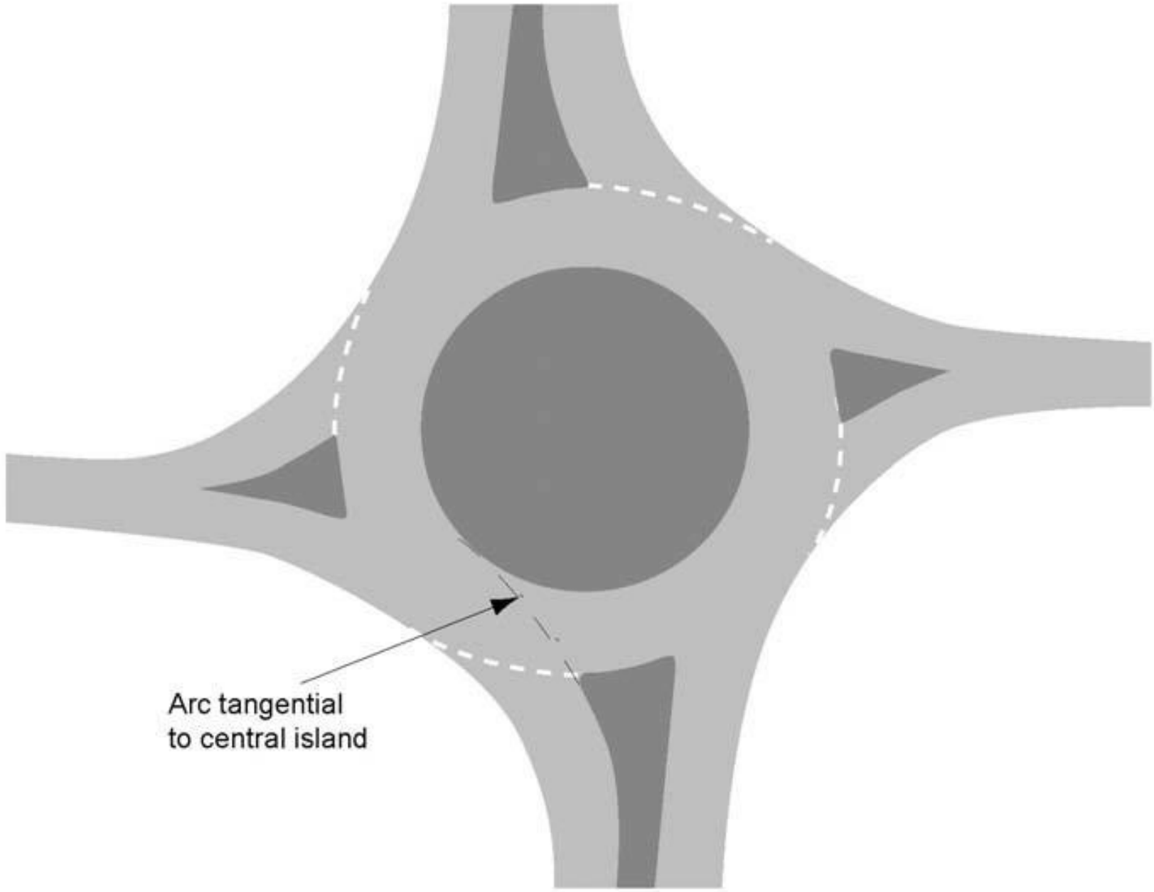
Figure 3.18.2 Example showing an arc projected forwards from the traffic island and tangential to the central island
