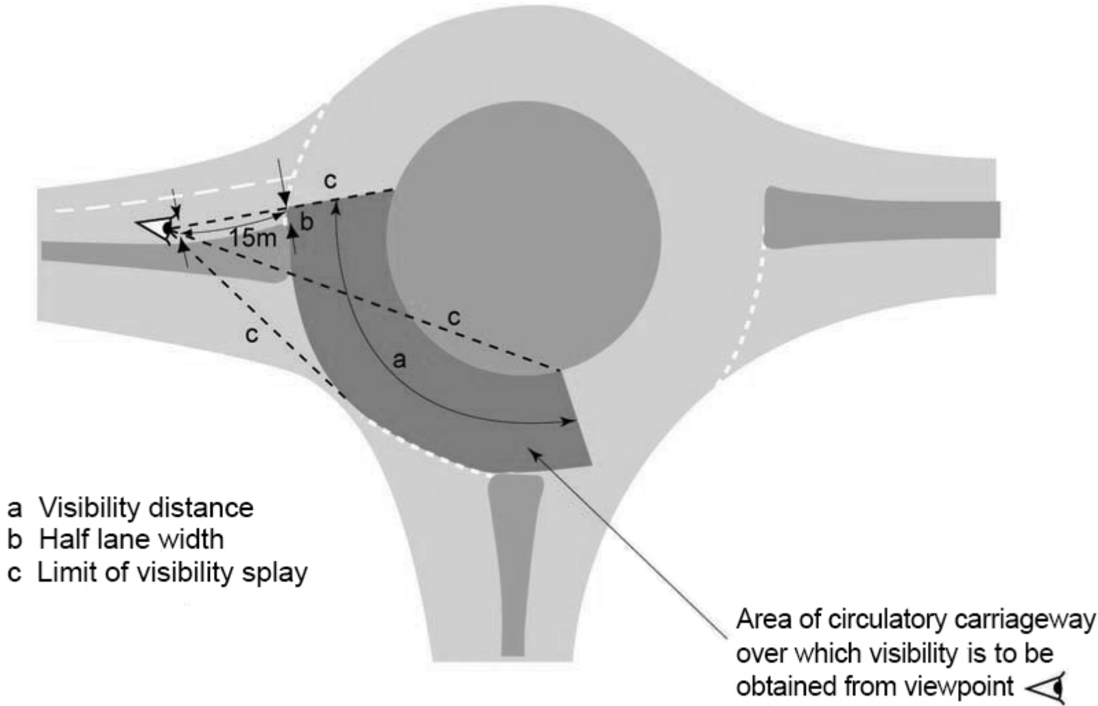
Figure 3.52 Visibility to right along circulatory carriageway measured at 15 metres in advance of give way line
