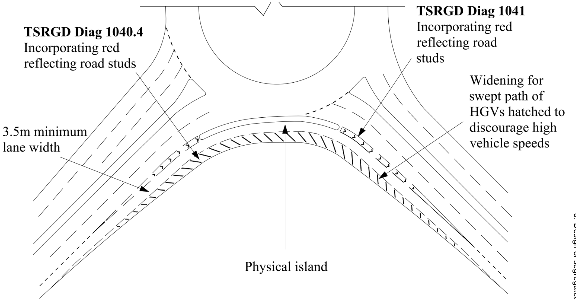
Figure 6.53.2b Generic physical segregated left turn lane
