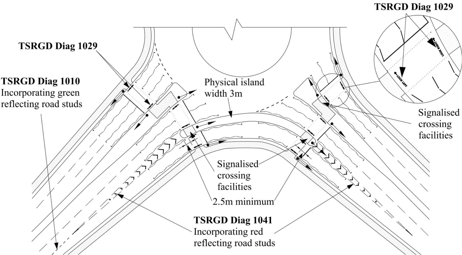
Figure 6.21 Physical SLTL with crossing facilities where pedestrians and cycle traffic are permitted (crossing facilities to be controlled)
