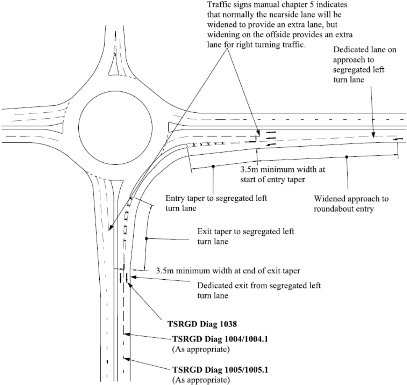
Figure 6.27N2a Dedicated approach and exit for SLTL
