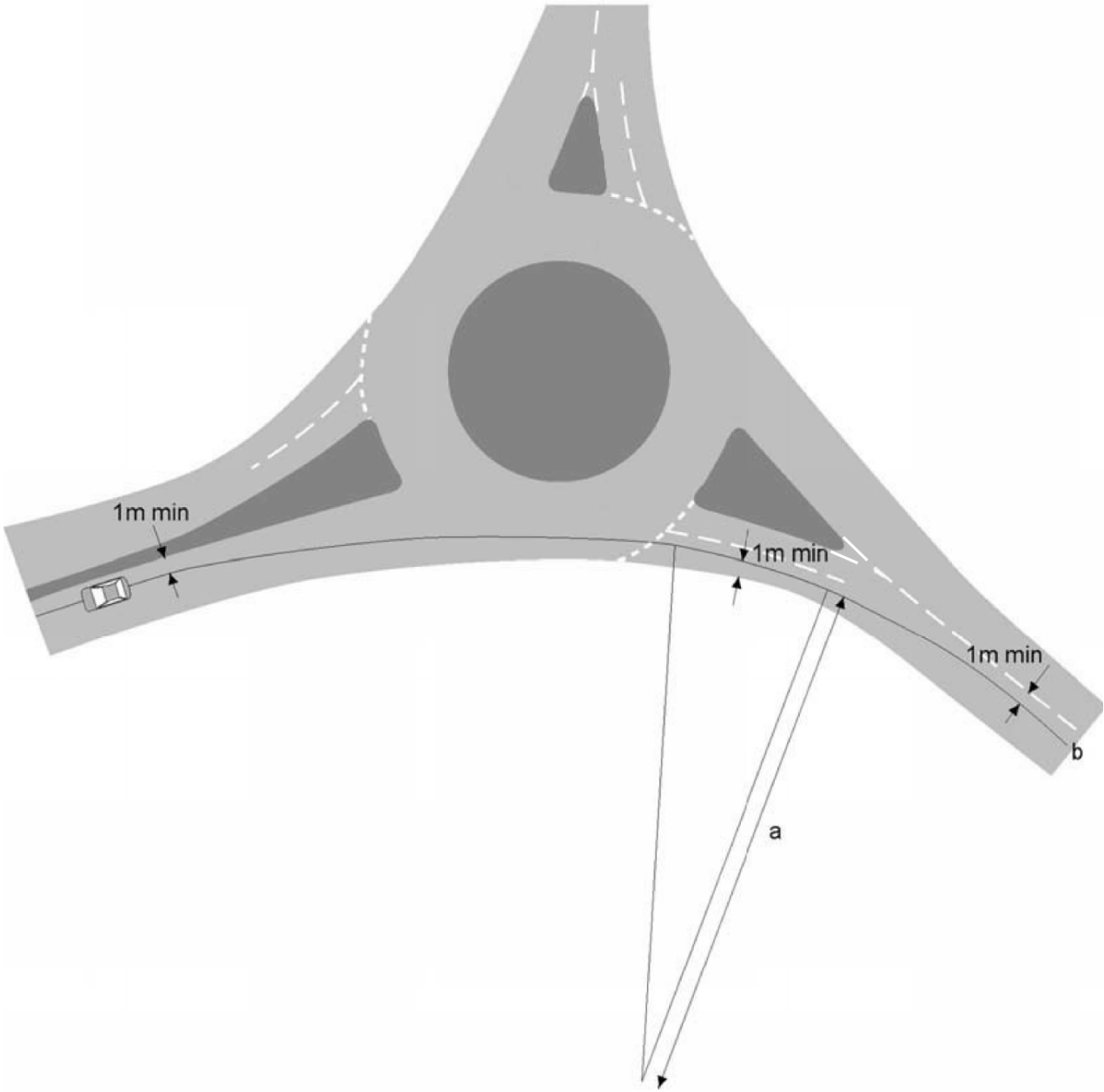
Figure A.1 Determination of entry path radius for the left turn at a roundabout at a Y-Junction
