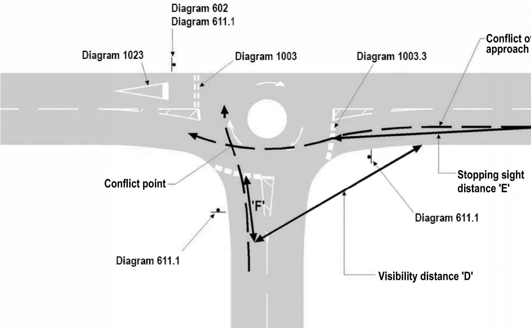
Figure 5.21 Mini-roundabout visibility distance 'D' and stopping sight distance 'F'
