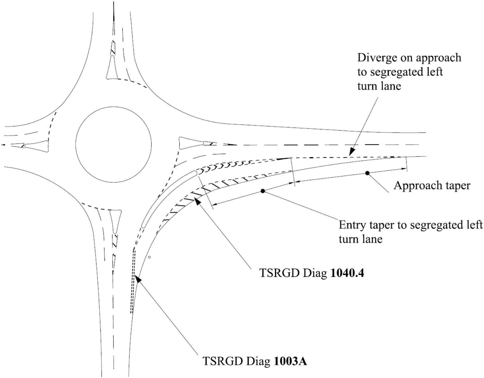
Figure 6.31 Physical SLTL approach taper
