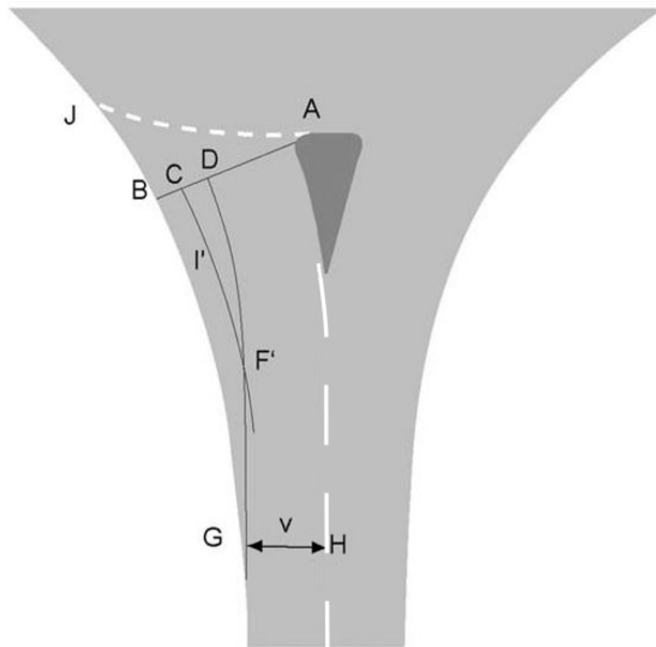
Figure 3.17 Average effective flare length
