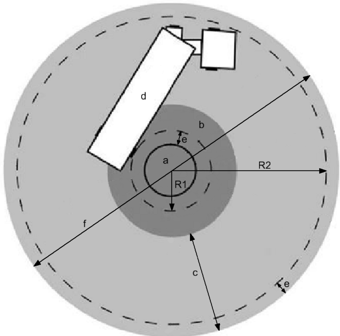
Figure 3.8.1N1 Turning widths required for compact or smaller normal roundabouts
