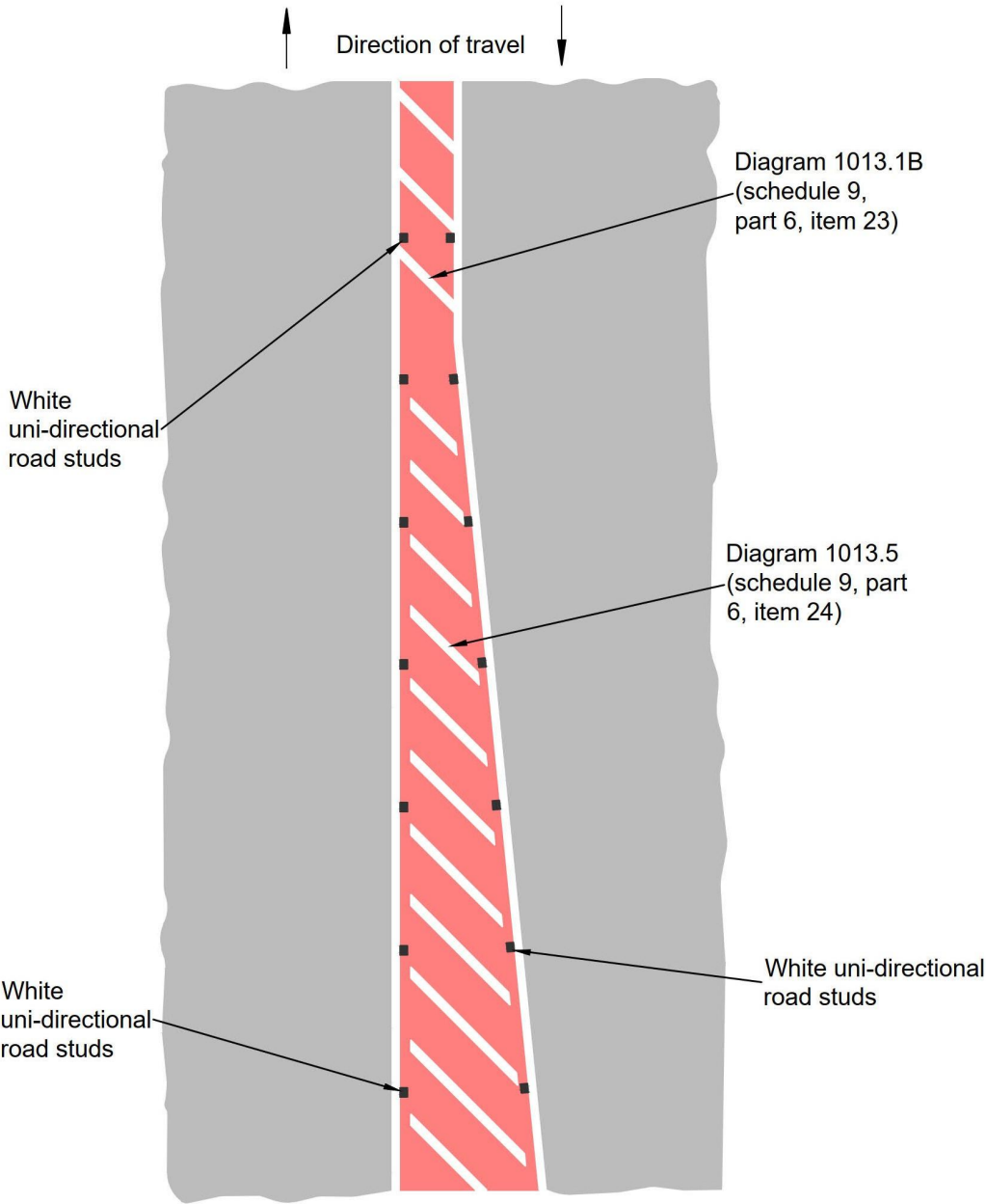
Figure 3.36 Interface between TSRGD diagram 1013.1B (schedule 9, part 6, item 23) and 1013.5 (schedule 9, part 6, item 24)
