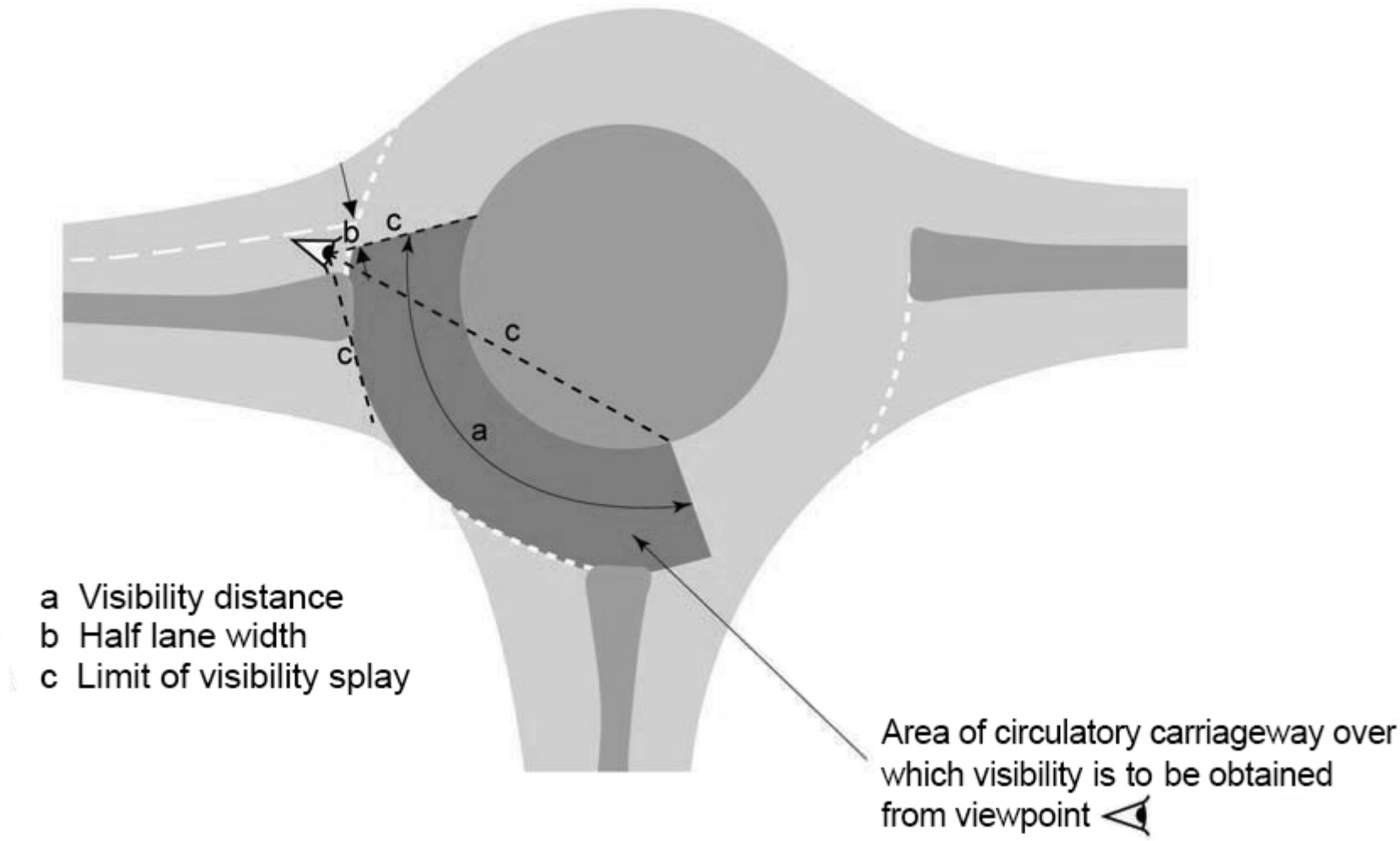
Figure 3.51 Visibility to right along circulatory carriageway measured at entry (from give way line)
